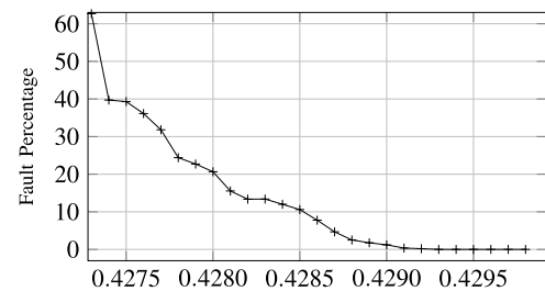
FIGURE 3. Percentage of faulty outputs at different supply voltages for a single sample chip.
