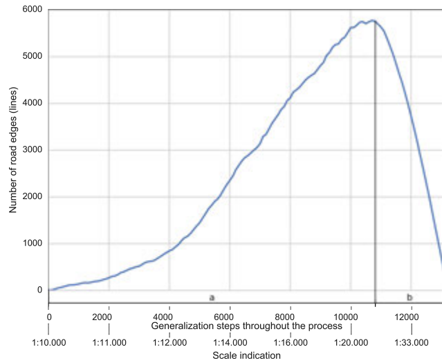
FIGURE 4.18 Number of road line edges in the structure (collapsed roads), related to Figure 4.12. Graph part a, where the number of collapsed road connections increases, represents the initial stage of the process, where roads are split/collapsed. Part b, where the graph decreases, indicates a situation where two area objects merge, intentionally removing the collapsed road lines between.
