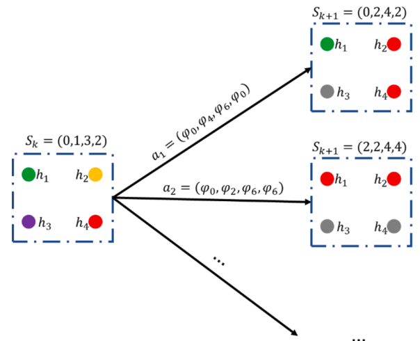
Fig. 4. An illustration of Markov decision process.
