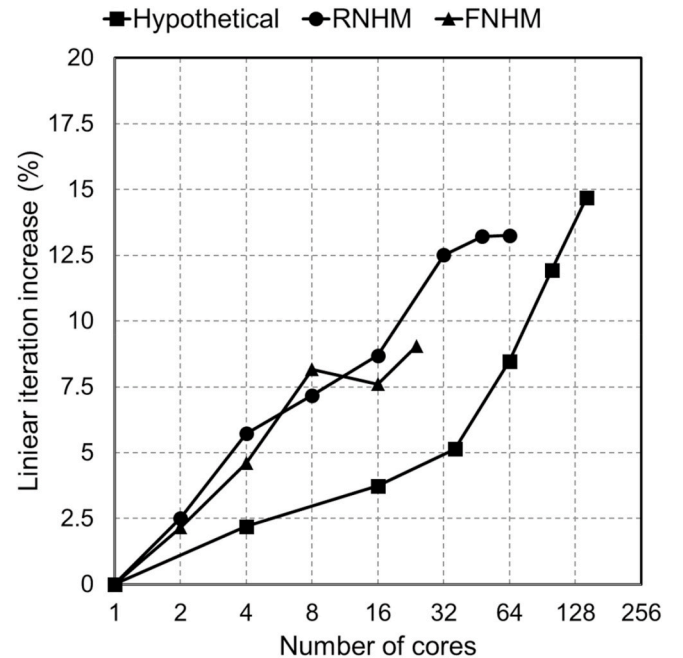
Fig. 8. Linear solver iteration increase for the hypothetical test case (3269 serial iterations), the reduced NHM (RNHM; 18,738 serial iterations) test case, and the fully-coupled NHM (FNHM; 30,390 iterations) test case.
