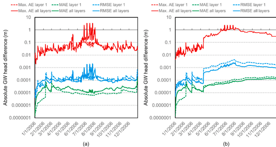
Fig. 11. Absolute groundwater head differences in meters for the reduced NHM test case (a) and the fully-coupled NHM test case (b), where for each test case a parallel run using 24 cores is compared to the reference serial run. Values are plotted for the top model layer and for all seven model layers. Max. AE: maximum absolute error; MAE: mean absolute error; RMSE: root mean squared error.
