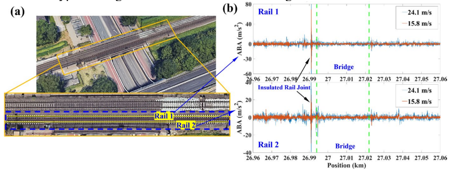
Fig. 2. Aerial photos of the transition zones and time histories of ABA measurements.
