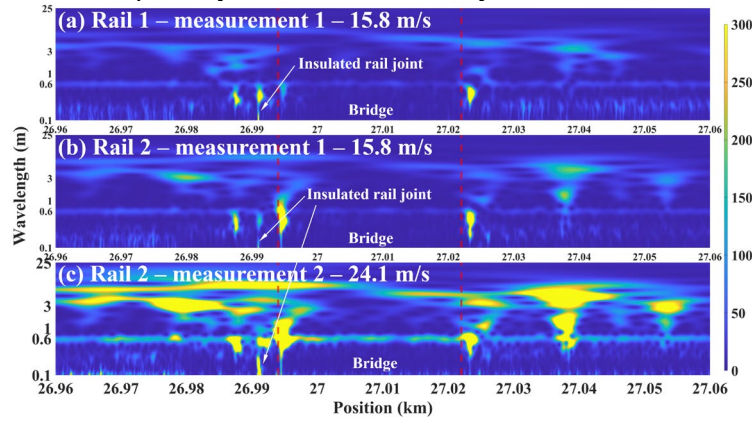
Fig. 3. WPS of the ABA measurements
