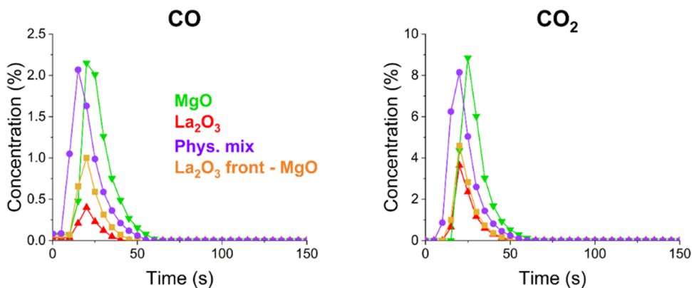
Figure 3. Transient analysis of products (FTIR + MS) during the \text{O}_2 pulse (0–150 s) in unsteady-state OCM performed at 900 °C. The values are averaged over multiple stable cycles of operation. Results for \text{La}_2\text{O}_3 (red \blacktriangle ), \text{La}_2\text{O}_3 -MgO 50 wt % physical mixture (violet \bullet ), MgO (green \blacktriangledown ), and \text{La}_2\text{O}_3 (10 wt %, front of the bed)-MgO (yellow \blacksquare ).
