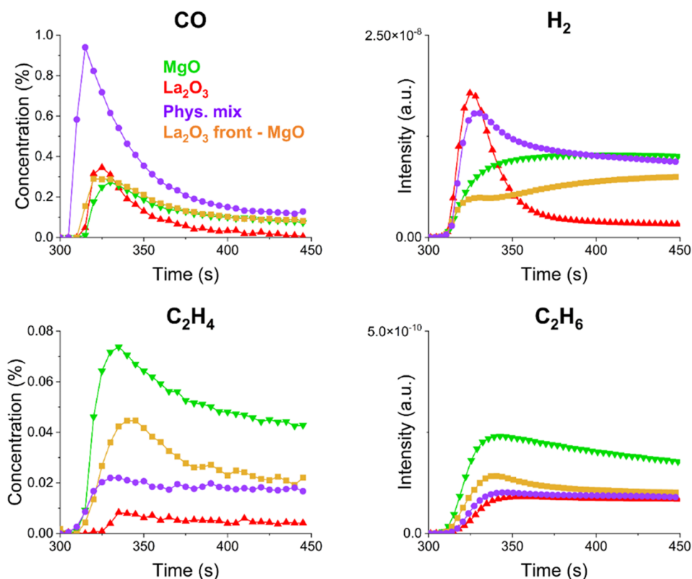
Figure 2. Transient analysis of products (FTIR + MS) during the \text{CH}_4 pulse (300–450 s) in unsteady-state OCM performed at 900 °C. The values are averaged over multiple stable cycles of operation. Results for \text{La}_2\text{O}_3 (red \blacktriangle ), \text{La}_2\text{O}_3 -MgO 50 wt % physical mixture (violet \bullet ), MgO (green \blacktriangledown ), and \text{La}_2\text{O}_3 (10 wt %, front of the bed)-MgO (yellow \blacksquare ).
