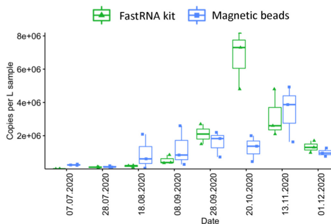
Fig. 5. Concentration of SARS-CoV-2 RNA in influent wastewater as determined by the average of N, ORF1ab and S gene assays in gene copies per L using two RNA extraction methods: FastRNA and MagMax (Magnetic beads) over the whole sampling campaign (July 2020 until December 2020) covering the second wave in The Netherlands.
