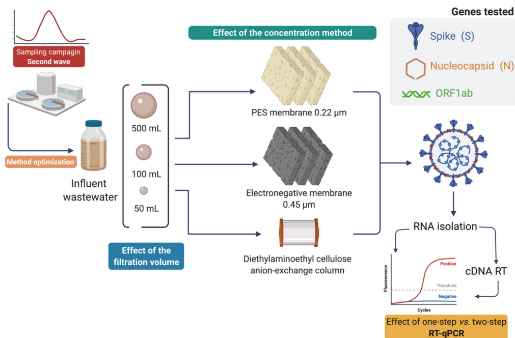
Fig. 1. Schematic representation of the experimental design followed in this study. Viral genes (S, N and ORF1ab) were quantified by RT-qPCR (one-step vs two-step RT-qPCR) after testing the effect of the filtration volume and different concentration methods. Created with BioRender.
