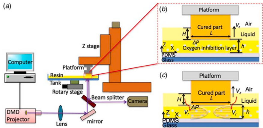
Fig. 4. Illustration of the mask video project-based stereolithography process [11].
