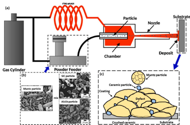
Fig. 13. The overview of the cold spray AM system using mixed powder [83].
