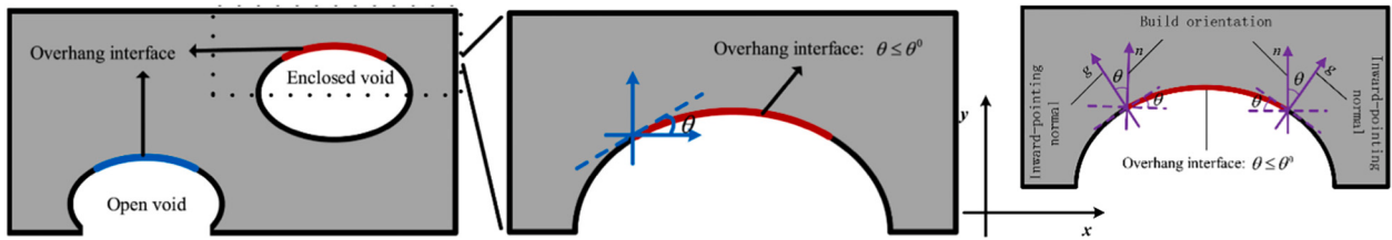
Fig. 9. Illustration of the overhang angle minimization approach [37].
