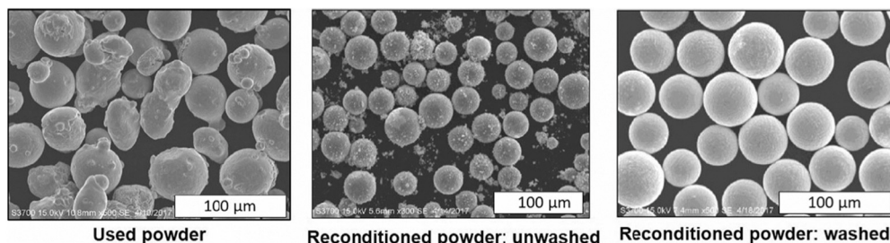
Fig. 18. Morphology of Inconel 718 particles at different states of reconditioning [116].
