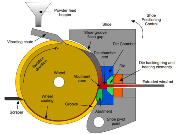
Fig. 19. Schematic of the Conform™ employed to produce wire feedstock directly from the recycled powder [118].
