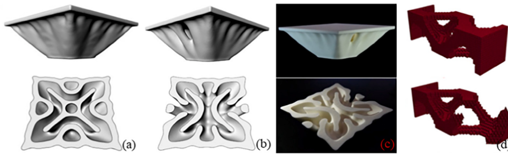
Fig. 7. Demonstrations of enclosed voids elimination (a) optimized structure, and (b) 3D printed structure [31] and void region restriction, (c) optimal design of a torsional beam, and (d) void restricted 3D printed parts (with/without supports) [32].
