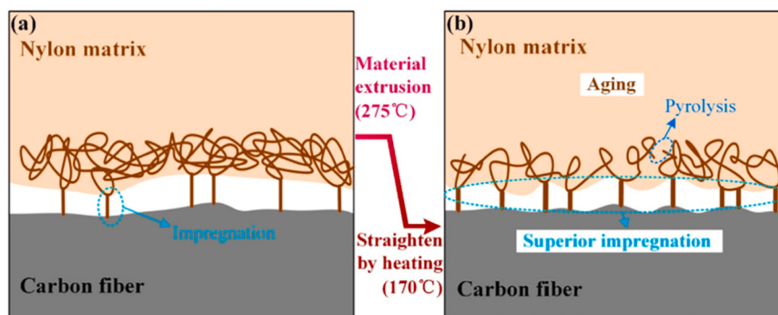
Fig. 20. Carbon fiber and Nylon interfacial bonds: (a) original composite and (b) recycled composite [123].
