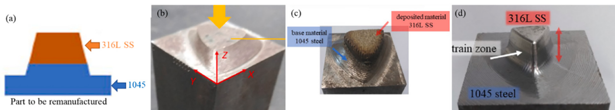
Fig. 15. Illustration of remanufacturing stages (a) Schematic of the part to be remanufactured, (b) AISI 1045 part after machining, (c) Restored part with 316LSS deposition, and (d) Final machined part [95].
