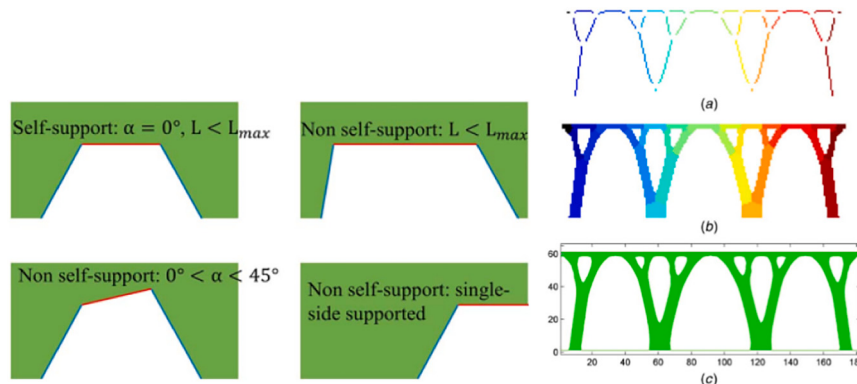
Fig. 8. Illustrations of (left) overhangs with close to zero inclination angle and (right) optimization results: (a) segmented structural skeletons, (b) segmented structural areas, and (c) self-support design [36].
