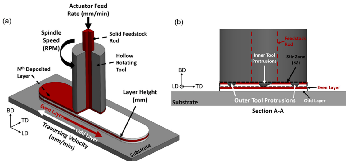
Fig. 14. (a) Illustration of FSAM process and (b) Toolhead interaction with the previously deposited layer [85].
