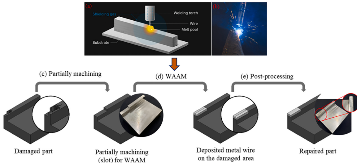
Fig. 12. Illustration of repairing damaged part using WAAM [78].
