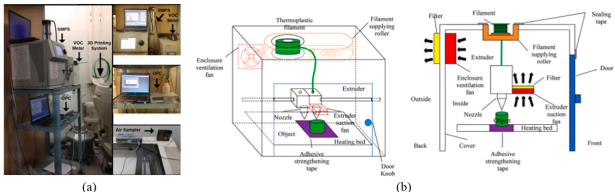
Fig. 10. Illustrations of emission measurement for (a) BJ [55]; and (b) FDM processes [58].
