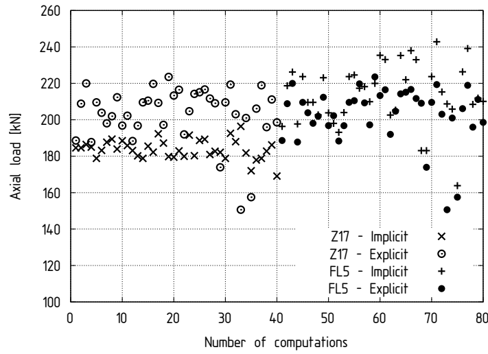
Figure 5: Stochastic studies - buckling load vs. number of computations - geometrical and lay-up imperfections - explicit vs. implicit dynamic analyses using Abaqus [14] and Ansys [13]
