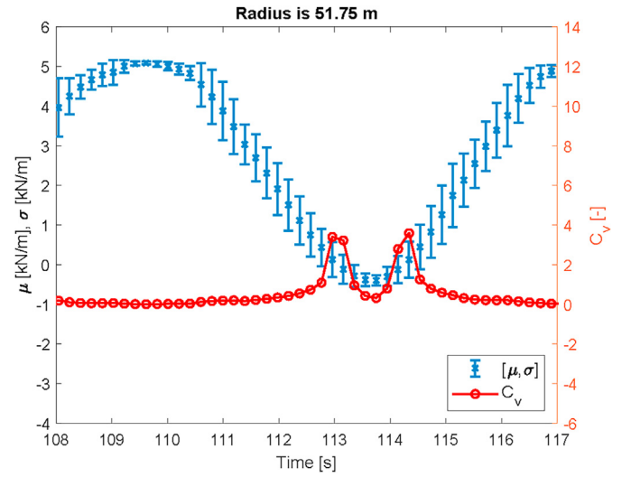
Fig. 27. The \mu , \sigma and C_v of dF_N at r = 51.75 m.
