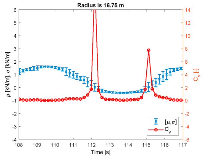
Fig. 23. The \mu , \sigma and C_v of dF_N at r = 16.75 m.
