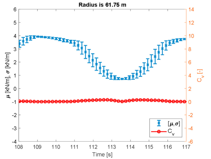
Fig. 28. The \mu , \sigma and C_v of dF_N at r = 61.75 m.
