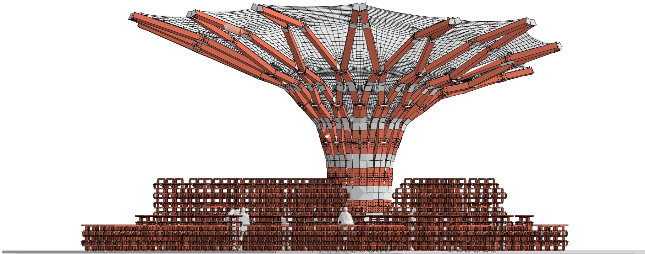
elevation : column : unfolded : with market : 1:100
