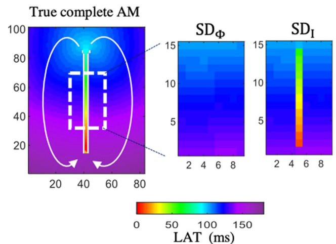
Fig. 6. Simulated tissue with two parallel vertical lines of block close to the center of the tissue that can potentially lead to a reentry circuit (denoted by white arrows). The white rectangle in the middle of the tissue denotes the location of the 15 \times 9 electrode array. The activation maps estimated using the steepest descent SD_\phi and our propose approach SD_I are also shown.
