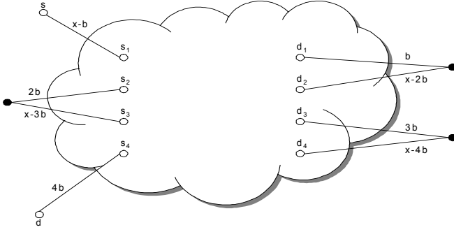
Fig. 3. Transformation of an MLBDP instance to an impairment-aware routing instance. Black nodes are regenerator nodes.
