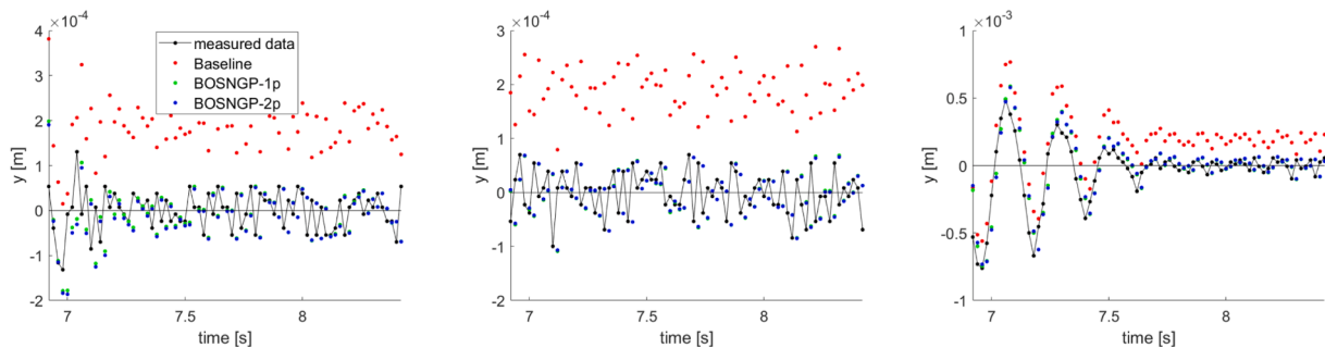
Fig. 10. The end phase of simulations carried out on the three test sequences of the magman problem. The last 1.5s of the simulations are shown.
