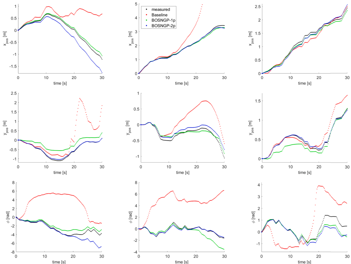
Fig. 9. Simulations with selected models of state variables x_{pos}, y_{pos} , and \phi on three test sequences of the turtlebot problem. Models with the test RMSE_{sim} value closest to the median value presented in Table 2 are selected for each state variable. From left to right are simulations on test 1, test 2, and test 3 data set.
