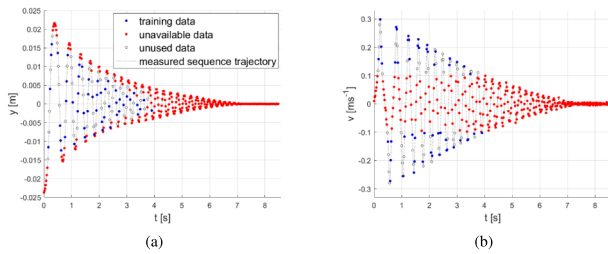
Fig. 7. Training data for (a) y and (b) v extracted from the data sequence measured for the first coil. Red dots are the samples with v < 0.1 \text{ ms}^{-1} , which are not considered for training. Out of the remaining samples, half of them are randomly selected for the training data set (the blue dots) leaving the other half unused (the black circles).
