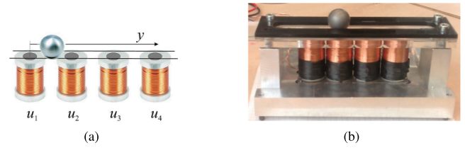
Fig. 6. Magman: A schematic (a) and a photo of the system (b).
