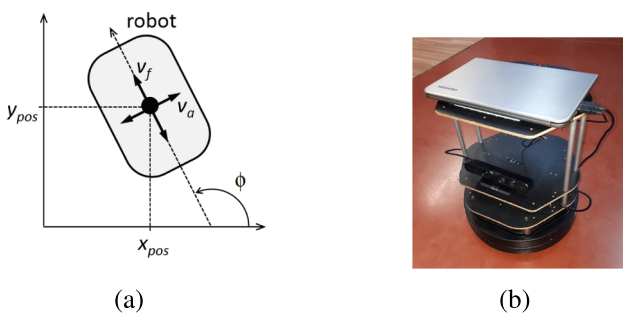
Fig. 4. TurtleBot mobile robot. A schematic (a) and a photo of the system (b).
