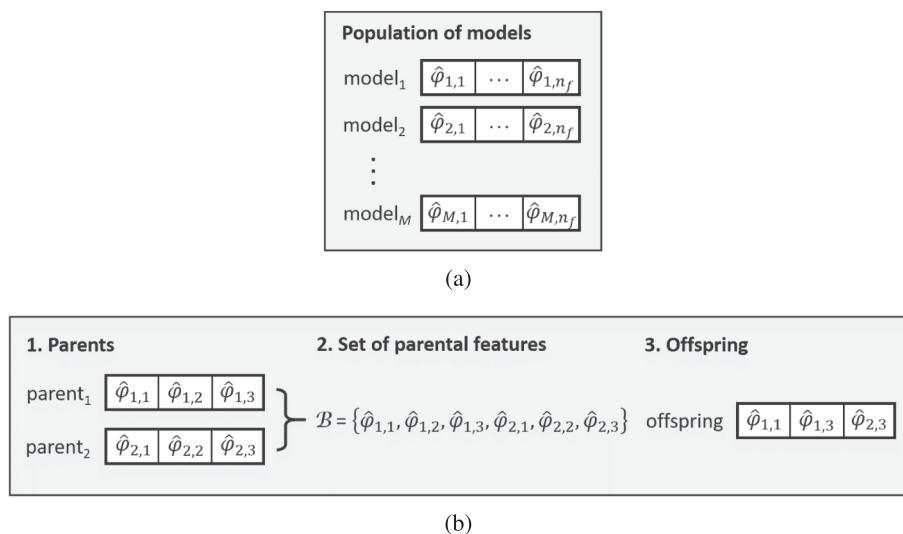
Fig. 2. (a) A population of models evolved in the feature mixing phase. Models are composed of encapsulated features, \hat{\varphi}_{ij} , that are immutable during this phase. (b) An illustration of the crossover operator used to create a new model as a combination of features of two parental models. The offspring model is composed of two features, \hat{\varphi}_{1,1} and \hat{\varphi}_{1,3} , inherited from the first parental model and one feature, \hat{\varphi}_{2,3} , inherited from the second parental model.
