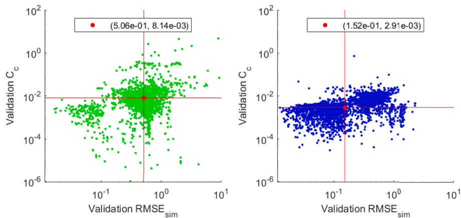
Fig. 8. A pool of all final models created for the state variable x_{pos} of the turtlebot problem in 50 runs of BOSNGP-1p and BOSNGP-2p. Green dots are models produced by BOSNGP-1p. Blue dots are models produced in the second phase of BOSNGP-2p. The median-median model is marked with the red dot.
