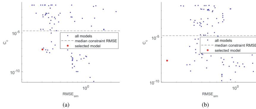
Fig. 3. Final model selection. (a) shows the case the selected model is a trade-off solution. (b) shows the case the selected model is an extreme solution. Both examples are from real experiments on the drone problem.
