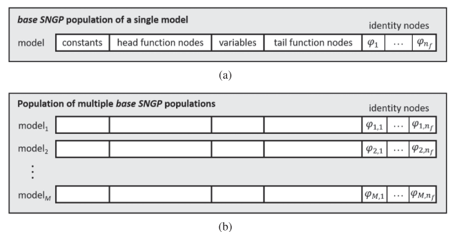
Fig. 1. Forms of the evolved population. (a) A population structure of the single-model base SNGP. (b) A multi-model population of multiple base SNGP populations.
