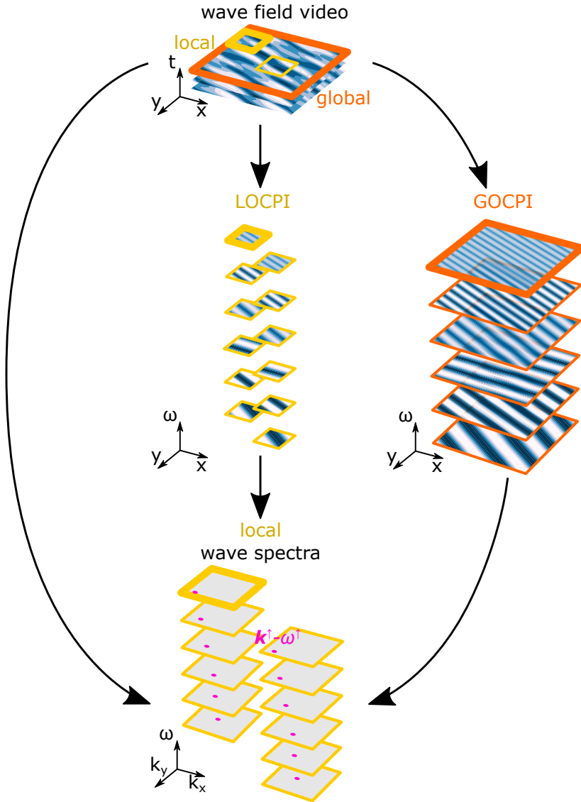
Figure 3.2.: Pathways to identify wavenumber-frequency signatures of gravity waves (k^\dagger, \omega^\dagger) (bottom panel, purple dots) in video of a wave field (top panel). The video can be transformed directly from space-time (x, y, t) into the spectral domain (k_x, k_y, \omega) (left pathway), or via construction of one-component phase images (x, y, \omega) , which may be local (LOCPI) (middle pathway) or global (GOCPI) (right pathway). In left and middle pathway all analyses are local (yellow). In the right pathway, the initial construction of GOCPI is global (orange) and then followed by local subdomain analysis to capture spatial variation in k^\dagger, \omega^\dagger .
