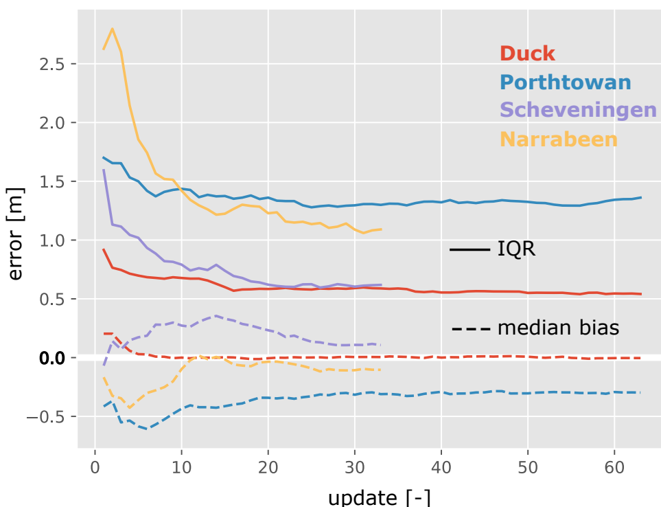
Figure 3.9.: Depth errors at successive updates for field sites Duck (red), Porthtowan (blue), Scheveningen (purple), Narrabeen (orange). Dashed lines present median bias. Solid lines present confidence intervals by the inter quartile range ( IQR = 75^{th} - 25^{th} percentile).
