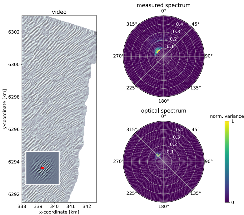
Figure 4.3.: Comparison of an in-situ measured (left, red 'x') variance density spectrum from a local buoy (top right) against a corresponding optical variance density spectrum from reconstructed satellite video (bottom right) of a representative area ( 2 \text{ km} \times 2 \text{ km} ) around the buoy location (left, white box). Both spectra are normalized to unit magnitude for comparison.
