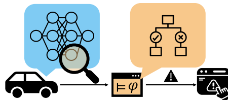
Figure 1: Runtime monitoring machine-learned controllers based on interpretable abstractions and reporting violations of the safety property \varphi to human operators.
