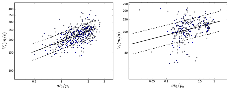
Fig. 4 Example of numerous V_S observations in the SCPT data set, for clays from the Peel Formation (left) and Naaldwijk Formation (right). The solid line describes the regression while dotted lines indicate 95% confidence intervals
