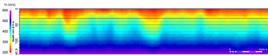
Fig. 10 Cross section through the MEI V_S model, from west to east at the centre of the field. The vertical scale is exaggerated
