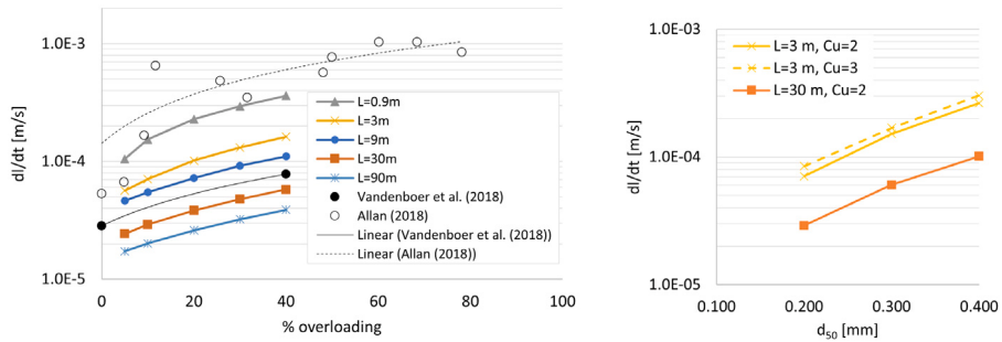
Allan (2018): d_{50} = 0.3 mm, L = 1.3 m. Vandenboer et al. (2019): d_{50} = 0.155 mm, L = 0.34 m.
