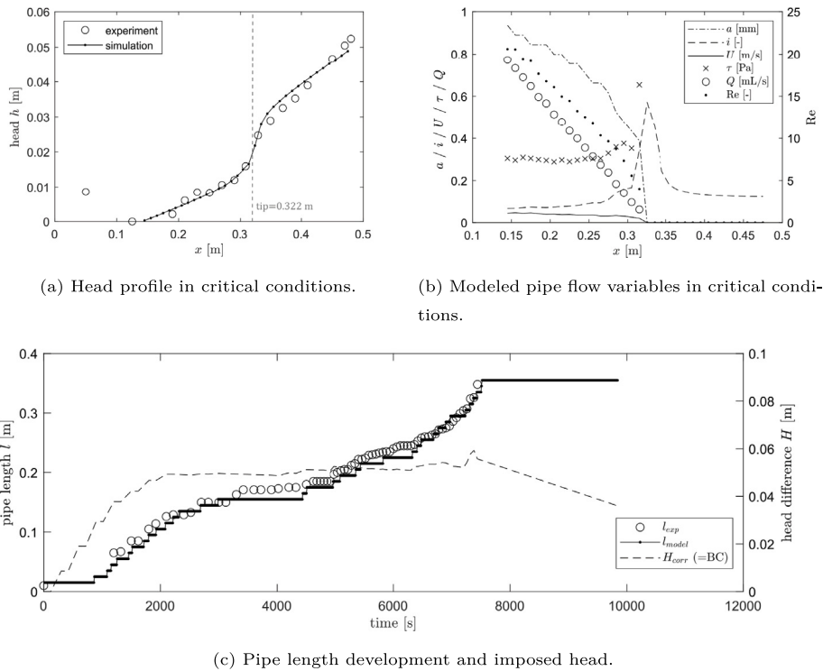
Fig. 5. Calibrated model results for small-scale experiment B25-245 ( i_{ip,c} = 0.9 , \eta = 0.3 , C_e = 0.014 ).
