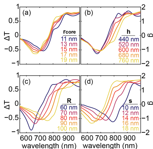
Figure 4. Simulation results of \Delta T versus wavelength for four geometrical parameter sweeps: radius of the core, r_{\text{core}} ; major radius R , height h , and gold shell thickness s . (a) Results for variation of the radius of the core, r_{\text{core}} . Five different radii were simulated, represented by different colors, while keeping other three geometrical parameters constant. (b) Variation of major radius R . (c) Variation of height h . (d) Variation of gold shell thickness s .
