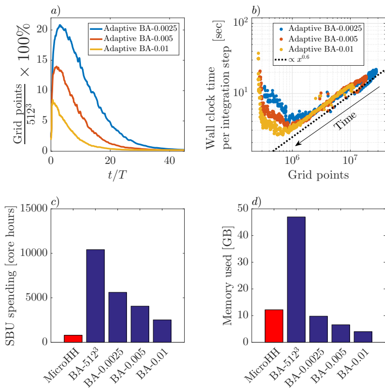
Figure 2.10: Overview of the performance characteristics of the adaptive and fixed-grid simulation runs. a) Time series of the number of grid points for the adaptive runs normalized by the maximum-resolution value (i.e. 512^3 ). b) Scatter plot of the wall clock time per integration step versus the used number of grid cells in the adaptive-grid runs. c) The total amount of System Billing Units (SBU, i.e. \text{number of cores} \times \text{hours} ) spending on each simulation run. Note that the value for BA-512 3 is estimated as if it were run until t/T = 45 . d) The total RAM memory used in each simulation run in gigabytes (GB).
