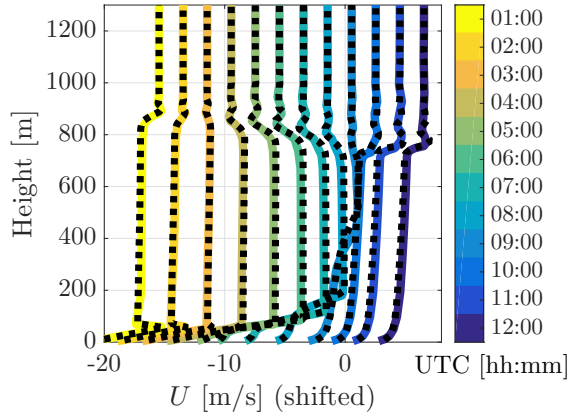
Figure 3.7: Vertical profiles of the wind-speed magnitude U obtained with the adaptive-grid (in colour) and the fixed equidistant-grid (dashed) SCMs. The twelve plotted profiles are obtained for the 24th of October with an hourly interval, starting from 1:00 AM local time. Noting that the profiles are shifted in order to distinguish between the different times (with vanishing wind at the surface). The profiles of U are constant with height for z > 1200\text{m} .
