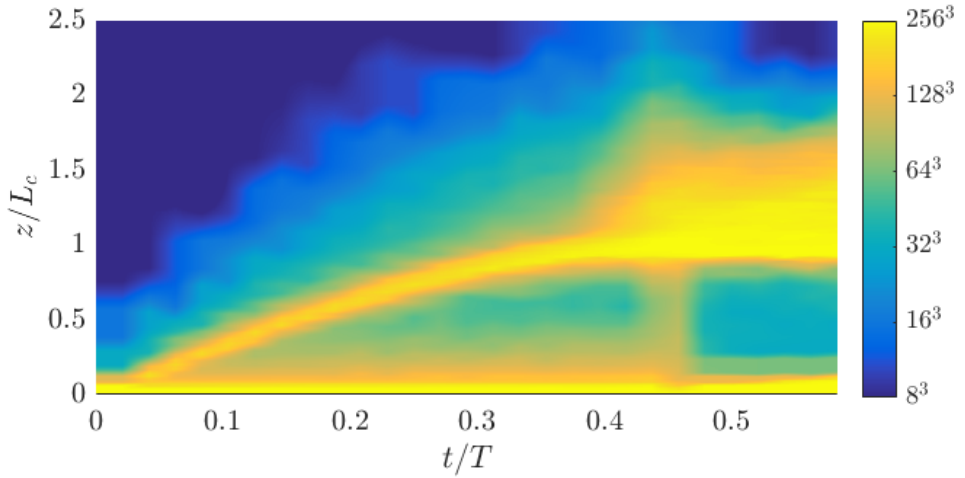
captionA1: The evolution of the equidistant-grid equivalent number of cells as a function of height (horizontally averaged).
