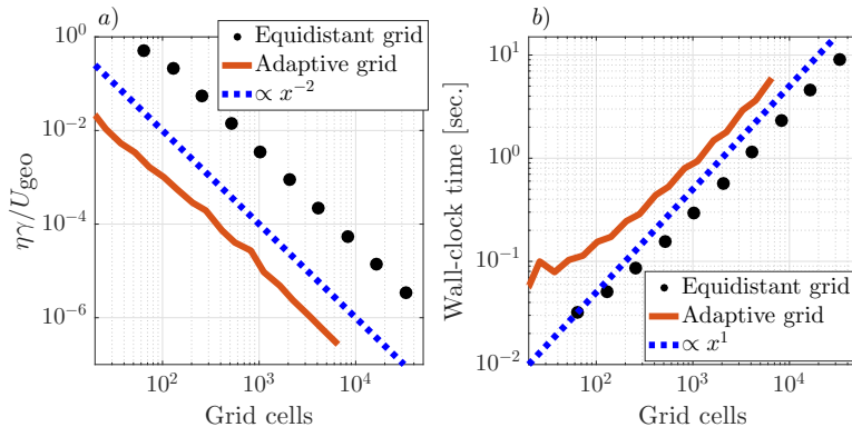
Figure 3.3: The scaling characteristics for the laminar-Ekman-spiral case. (a) Presents the error convergence for the equidistant-grid and adaptive-grid approach. The errors ( \eta ) follow the slope of the blue dashed line that indicates the second-order accuracy of the methods. The wall-clock time for the different runs is presented in (b), showing that for both of the aforementioned approaches, the required effort scales linearly with the number of grid cells.
