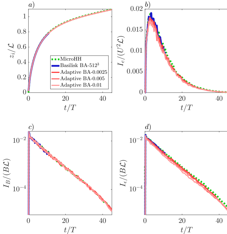
Figure 2.8: Time series of the domain integrated quantities, a) boundary-layer height ( z_i ), b) kinetic energy ( I_e ), c) buoyancy flux ( I_B ) and d) dissipation rate ( I_\epsilon ) according to Eq. 2.11. The results are obtained with both Basilisk and MicroHH using fixed grids and Basilisk using the adaptive mesh refinement algorithm. Note that plots c) and d) use a logarithmic scale.
