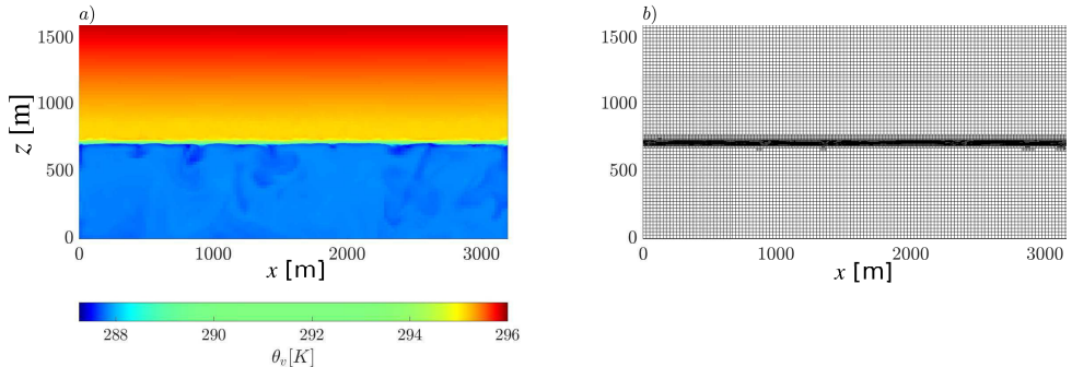
Figure 2.11: Snapshots of a) the vertical slices of the virtual potential temperature field and b) the numerical grid at t = 3 h. The case is based on the work of Bretherton et al. (1999).
