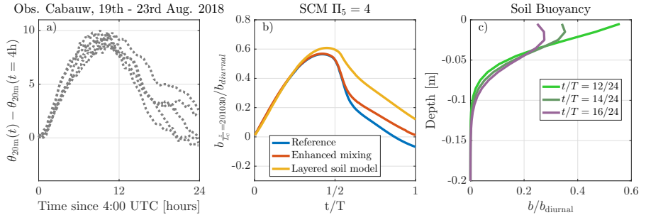
Figure 4.7: The evolution of the temperature at z = 20 m for five consecutive clear-sky and relatively dry days with a pronounced diurnal pattern, at Cabauw, The Netherlands (a) and the modeled buoyancy at z = L_c/50 \equiv 20 m obtained from three different models (b, see text Sect. 4.3). It appears that at the onset of the stable boundary layer ( t \approx T/2 ), only the model that includes heat-storage effects (yellow line) is able to predict a realistic cooling rate. The corresponding soil-buoyancy profiles (c) are displayed for various times during the day-to-night transition. These profiles reveal that after the transition, the soil is releasing heat into the atmosphere.
