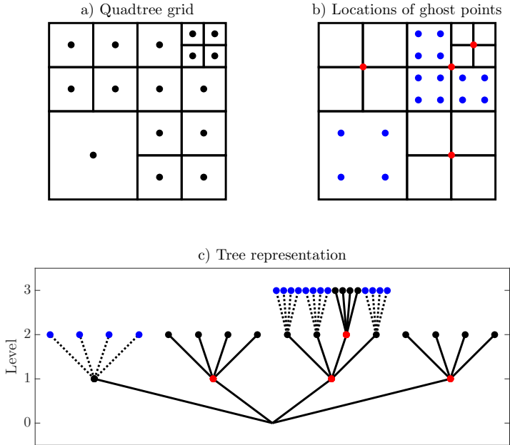
Figure 2.2: Example of a tree-grid structure. The top row presents the spatial structure of the grid cells with varying levels of refinement (a) and the locations of two types of ghost points whose field values are defined by the downsampling (red dots) and upsampling (blue dots) operations (b, see text). The plot on the bottom row presents a corresponding tree representation of the various grid cells and ghost points at different levels (c).
