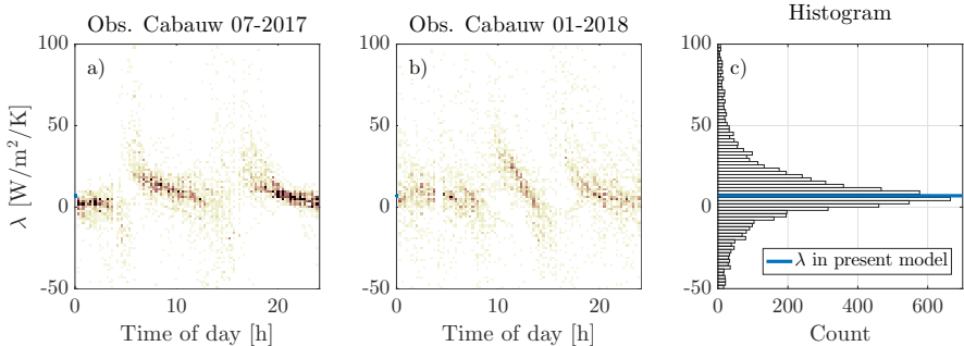
Figure 4.1: Population-density plot of estimated \lambda values based on observations taken at the CESAR site, in Cabauw, The Netherlands. The plot reveals that \lambda is highly variable and shows characteristic behavior with respect to the time of day. c) shows the histogram of all shown \lambda values.
