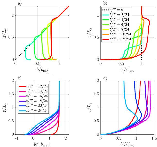
Figure 4.4: The solution profiles obtained for the single-column model run with \Pi_5 = 3.5 . The plots display the profiles of the daytime the buoyancy ( b ) and the horizontal wind magnitude ( U ) in panel a and b, respectively. Panels c) and d) display the same quantities for the nighttime. Notice the different scaling of the axis for daytime and nighttime data. For reference; all panels show the corresponding profile at t = T/2 (red line).
