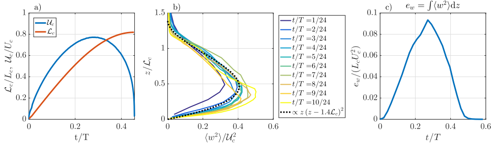
Figure 4.10: The time evolution of the CBL height ( \mathcal{L}_c ) and the instantaneous convective velocity scale ( \mathcal{U}_c ) according to Eqs. 4.29 and 4.30 (a), the vertical ( z ) profiles of the velocity variance \langle w^2 \rangle , plotted for different times and normalized with the external scales \mathcal{L}_c and \mathcal{U}_c , respectively, (b). The dashed black line indicates a fit (by eye) of a functional relation for the self-similar profile based on (Troen and Mahrt, 1986). The growth and the subsequent decay of the resolved turbulent motions are quantified by the total height-integrated vertical velocity variance ( e_w ) (c).
