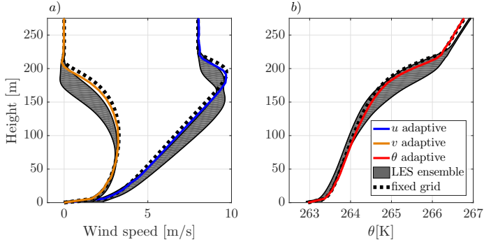
Figure 3.4: Time averaged profiles over the ninth hour of the run according to the GABLS1 intercomparison scenario. For (a) the horizontal wind components and (b) the potential temperature. Results are obtained with the present adaptive-grid SCM (coloured lines), the LES models ensemble (i.e mean \pm \sigma ) from Beare (2006) (grey-shaded areas) and the present SCM, employing an equidistant and static grid with a 6.25 meter resolution (dashed lines). For z > 250\text{m} , the profiles have remained as they were initialized.
