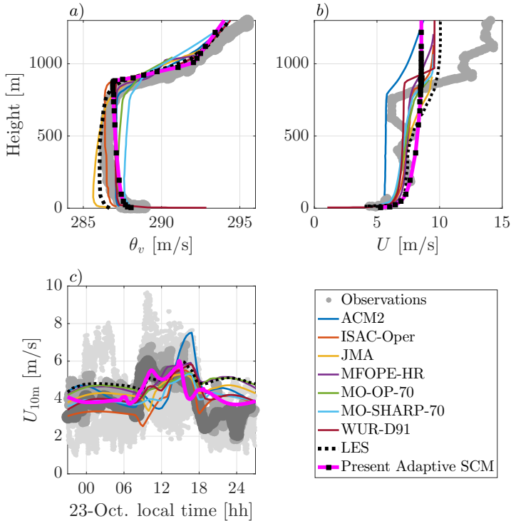
Figure 3.6: Comparison of the results obtained with the adaptive-grid SCM and the participating models in the work of (Svensson et al., 2011) for the vertical profiles of (a) the virtual potential temperature and (b) the wind-speed magnitude, for 14:00 local time on the 23rd of October. Lower panel: (c) the evolution of the 10-meter wind speed ( U_{10m} ) on the 23rd of October. For the used model abbreviations in the legend, see Svensson et al. (2011). The different shades of grey in plot c) indicate observations from different measurement devices, see Svensson et al. (2011) for the details.
