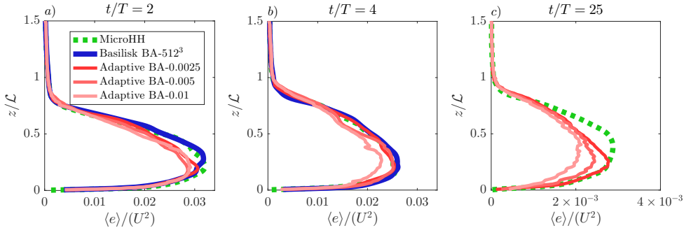
Figure 2.9: Vertical profiles of the horizontally-averaged kinetic energy ( \langle e \rangle ) at t/T = \{2, 4, 25\} in left, middle and right plot, respectively. The results are obtained with both Basilisk and MicroHH using fixed grids and Basilisk using the adaptive mesh refinement algorithm. Note that in panel c) the horizontal axis is rescaled and that regular-grid computations with Basilisk are not available (see text, Sect. 2.2.4).
