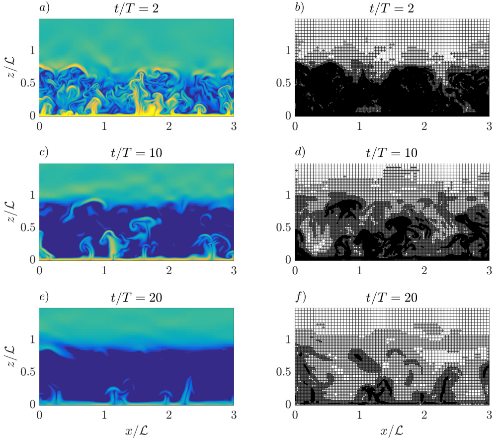
Figure 2.7: Vertical slices of the \|\nabla b\| field (left column) and the corresponding numerical grid (right column) in the lowest half of the domain. The top, middle and bottom rows represent snapshots taken at t/T = \{2, 10, 20\} , respectively. These snapshots are taken from the adaptive-grid run BA-0.0025.
