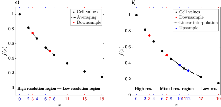
Figure 2.4: Example of the treatment of a resolution boundary in a one-dimensional scenario. First, the high level region near the resolution boundary is downsampled to obtain values for the coarse-level ghost points in red (a). Second, linear interpolation of the coarse level solution is used to define the field values of high level ghost points in blue (b).
