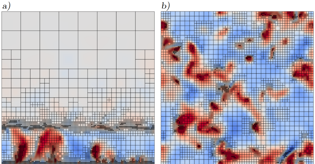
Figure 4.12: A2: A vertical (a) and a horizontal slice (b) of the vertical velocity (color) and the used adaptive-grid structure. These slices are taken over the full domain at t/T = 6/24 and the horizontal slice is obtained at height z = L_c/3 .
