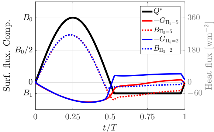
Figure 4.5: The diagnosed buoyancy flux ( B ), the soil heat flux ( G ) and the prescribed net radiation ( Q^* ) obtained from two runs, each with different \Pi_5 value ( \Pi_5 = \{2, 5\} ). The differences due to the wind forcing are most notable in the stable boundary layer regime (i.e. t > T/2 ). After the occurrence of a buoyancy flux minimum, the sensible heat flux vanishes for the case with the weaker wind forcing, whereas it remains finite for the case with the stronger forcing case.
