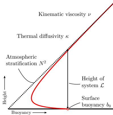
Figure 2.6: Sketch of the system and its parameters. The red line illustrates a typical buoyancy profile within the CBL during the initial development. Adapted from Van Heerwaarden and Mellado (2016).
