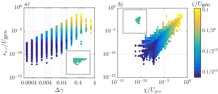
Figure 3.2: The locally evaluated error in the numerical solutions for u and v at t = t_{\text{end}} , based on the analytical solution ( \epsilon_{u,v} , see Eq. 3.23) for 20 runs using the adaptive-grid approach with different refinement criteria (see colour bar). The left-hand side plot (a) Shows that the diagnosed errors for each run plotted against the used mesh-element size ( \Delta ). The inset (using the same axis scales) shows the results for a single run. The right-hand side plot (b) shows the correlation between the wavelet-based estimated error ( \chi ) and the corresponding diagnosed error in the numerically obtained solution ( \epsilon ). The inset (using the same axis scales) shows the results for a single run, and reveals a relatively small spread in both \epsilon and \chi values compared to the equidistant-grid results presented in figure 3.1b.
