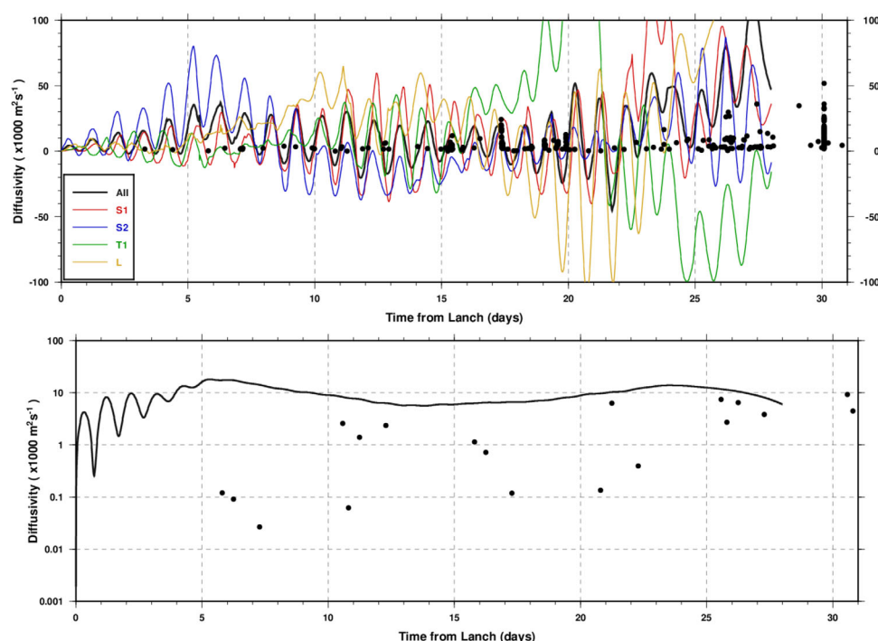
Figure 13. (top) The horizontal diffusivity K , in 10^3 \text{ m}^2/\text{s} , as a function of time after deployment in days for the primary drifter clusters. Note that the smallest and largest values fall outside the axis limits here. The minimum and maximum values of K are from cluster L and are -110 \times 10^3 \text{ m}^2/\text{s} and 360 \times 10^3 \text{ m}^2/\text{s} , respectively. The dots show the horizontal diffusivity calculated by Taylor's method as described in the text. (bottom) The solid line in this plot is a spline-smoothed version of the ALL curve from the top figure on a log scale. The dots are an average of all of the Taylor-based estimates for each of the temporal midpoints of the 31 day data segments.
