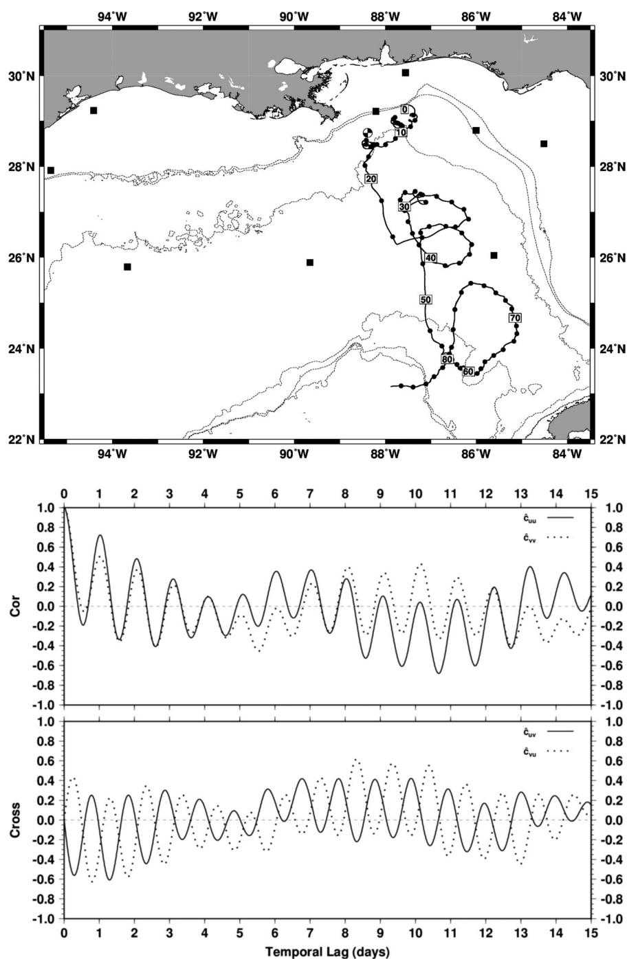
Figure 4. (top) The 85 day trajectory of drifter 218 deployed on 29 July 2012 near the shelf break. It sampled different dynamical regimes from slow flow dominated by inertial motion near the shelf break to faster mesoscale flow in the deeper Gulf of Mexico. The dots are plotted daily, and the number denotes days since deployment. The 200 m, 300 m, and 2000 m isobath contours are also plotted. The 9 black squares are the locations of the National Data Buoy Center (NDBC) moored stations. The Deepwater Horizon site is denoted by the black-white circle. Below the trajectory plots are the (middle) horizontal velocity autocorrelation and (bottom) cross correlation functions for two different 30 day segments for u and v . Drifter 218 velocity autocorrelation and crosscorrelation are calculated for the first 30 days of the trajectory in the middle plot, while the bottom plot is for the last 30 days of the trajectory. The solid and dotted lines in the upper part of the middle and bottom plots are \hat{C}_{uu} and \hat{C}_{vv} , respectively. The solid and dotted lines in the lower part of these plots are \hat{C}_{uv} and \hat{C}_{vu} , respectively.
