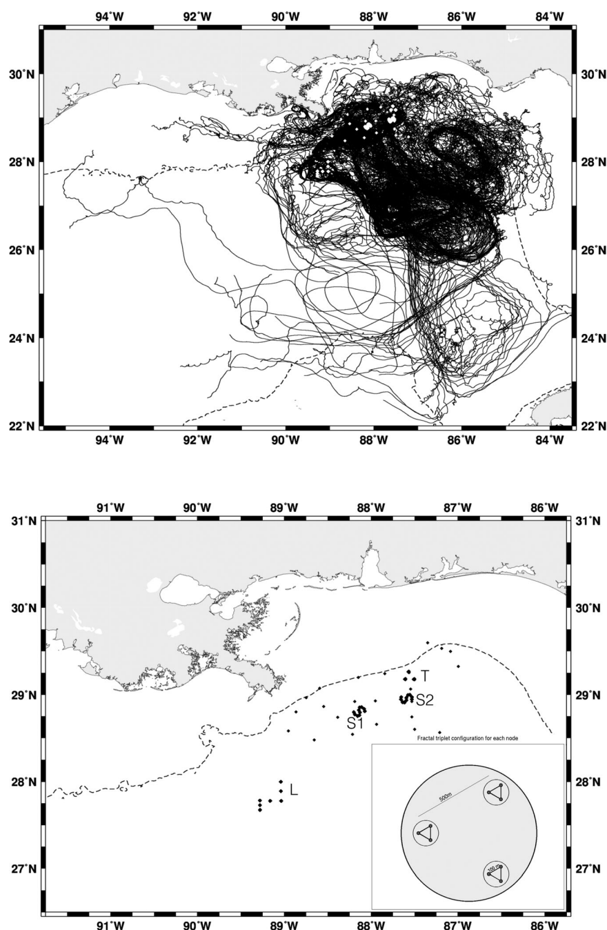
Figure 1. (top) Spaghetti plot of the GLAD drifters used in this analysis. The black lines are the GLAD drifter trajectories that are mostly 2–3 months in length. The 300 m isobath contour is shown as a dashed line, land and the launch locations, primarily offshore of 300 m depth and near 89°W, 28°N, are plotted in shades of grey for the northern GoM. The coastline of Louisiana, Mississippi, Alabama, and the western Florida “panhandle and Big-Bend region” are visible in the north, as well as parts of western Cuba in the southeast corner of the plot. (middle) The details of the survey launches, S1, S2, L, and T deployments with larger diamonds implying nodes. The inset is the deployment pattern of the nodes consisting of 3 sets of triplets spaced 500 m apart with 100 m spacing for the triplets. (bottom) The average position for all of the 31 day data segments used for analysis are plotted.
