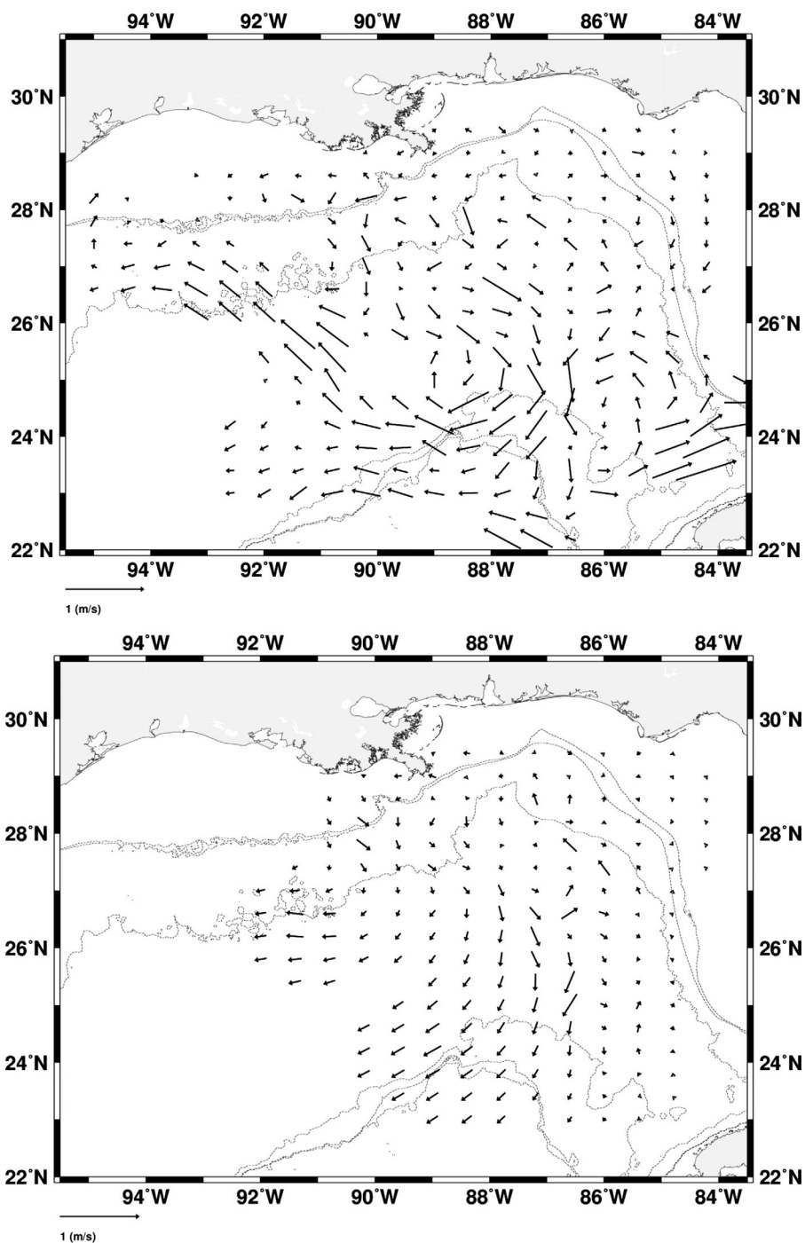
Figure 2. Lagrangian estimate of the average surface velocity during the GLAD experiment in the northern Gulf of Mexico using (top) 10 day data segments and (bottom) 31 day data segments. The 200 m, 300 m, and 2000 m isobath contours are also plotted.
