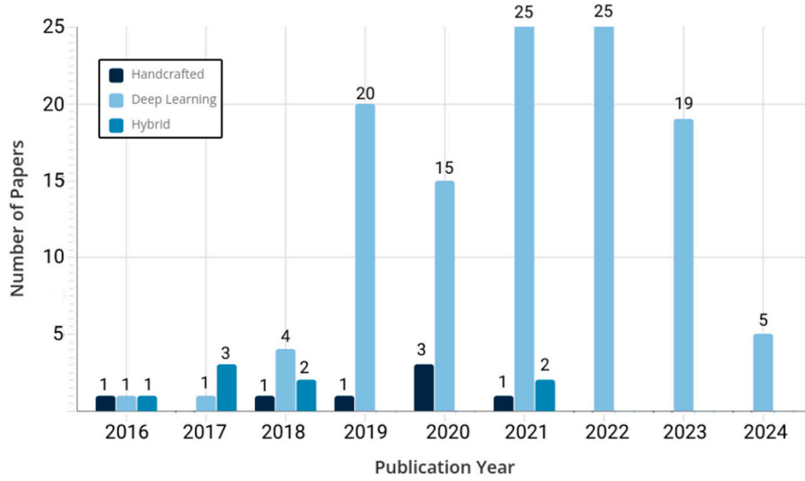
Fig. 7. The trends of employing various approaches explained in this survey by state-of-the-art research works published in different years (2016–2024).
