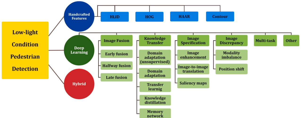
Fig. 5. The primary classification of different nighttime pedestrian detection methodologies considered in this survey.
