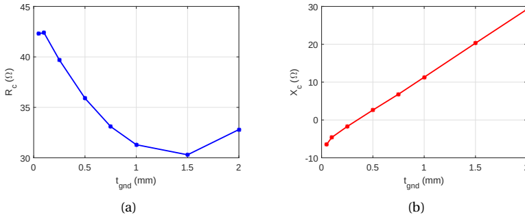
Figure 9.29: Active impedance of a center element at f_0 with varying t_{\text{gnd}} for L_{\text{max}} = 5\lambda_0 , L_p = 3.20 \text{ mm} , W_p = 2.50 \text{ mm} , (a) resistance, (b) reactance.
