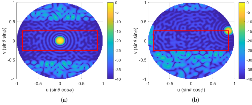
Figure 10.26: Radiation pattern at f_0 (normalized w.r.t. broadside gain, in dB) of the 256-element, fully aperiodic array with d_{\min} = 0.5\lambda : (a) broadside beam, (b) corner beam.
