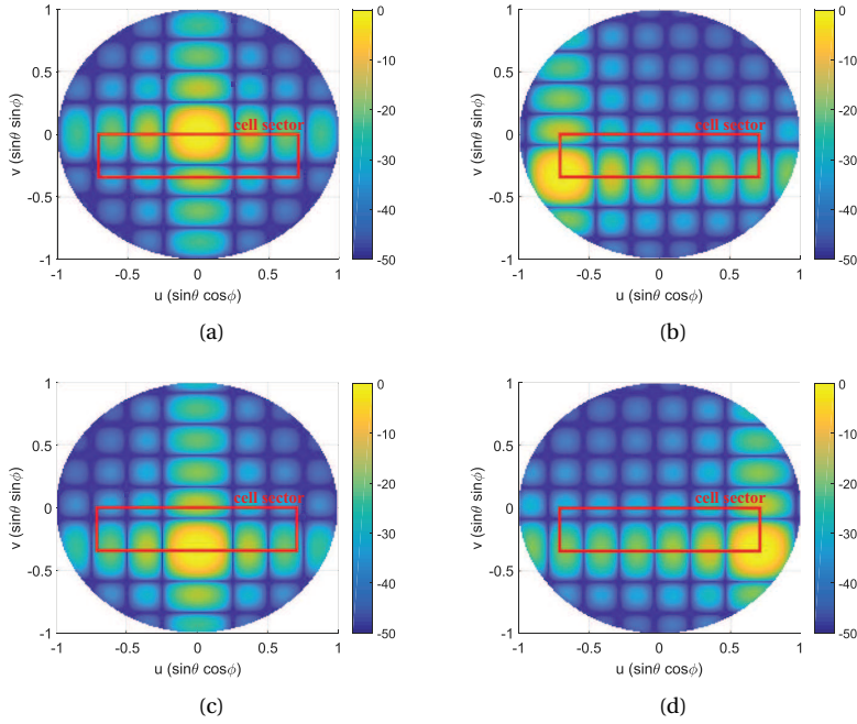
Figure 6.17: Multi-beam radiation patterns (in dB, normalized) for the test case with the regular array for a beam scanned towards (a) u_{s1} = v_{s1} = 0 , (b) u_{s2} = -\sin(\pi/4) , v_{s2} = -\sin(\pi/9) , (c) u_{s3} = 0 , v_{s3} = -\sin(\pi/9) , (d) u_{s4} = \sin(\pi/4) , v_{s4} = -\sin(\pi/9) .
