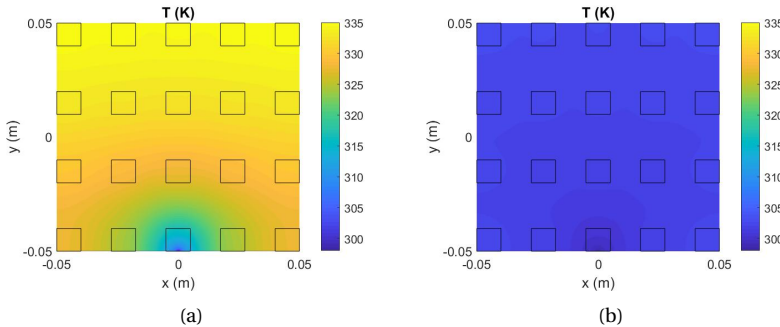
Figure 9.2: Temperature field results from CST MPS for uniform distribution (UD) of 20 heat sources in Case 1 and Case 4: (a) UD, Case 1 (no emission), (b) UD, Case 4 (with \varepsilon = 0.1 ).
