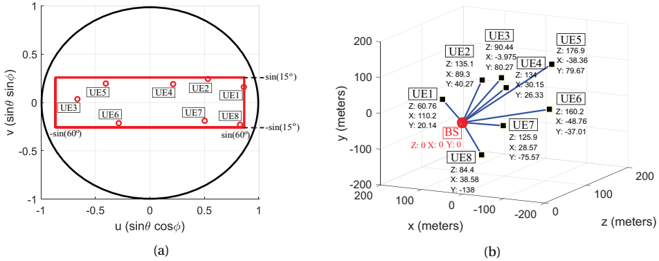
Figure 2.19: A sample distribution of 8 random users/relays at different heights with interference-aware selection in Use Case B in (a) uv -plane, (b) Cartesian coordinates.
