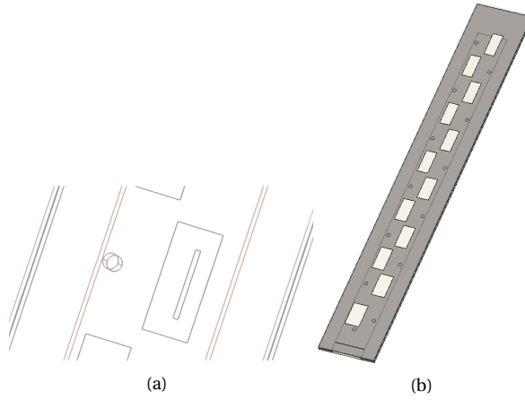
Figure 5.8: Illustration of the SIW-fed horizontally polarized AC-MPA subarray: (a) a single element in the array, (b) the complete subarray.
