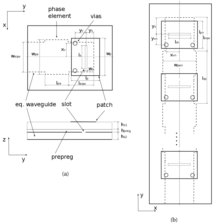
Figure 10.1: Geometry of the SIW-fed AC-MPA subarray.
