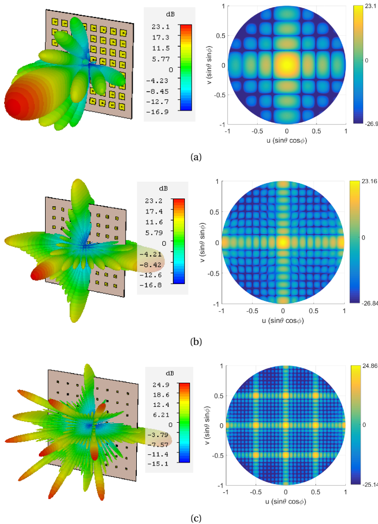
Figure 9.12: Realized gains of 8x8 regular square array layouts for broadside beams at 28.5 GHz, (a) d_e = 0.5\lambda , (b) d_e = 1\lambda , (c) d_e = 2\lambda .
