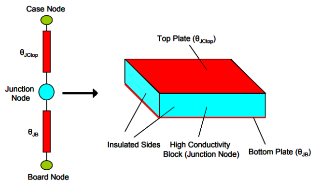
Figure 8.4: Representation of two-resistor model in a simulation environment via a block-and-surface resistance approach (taken from [163]).
