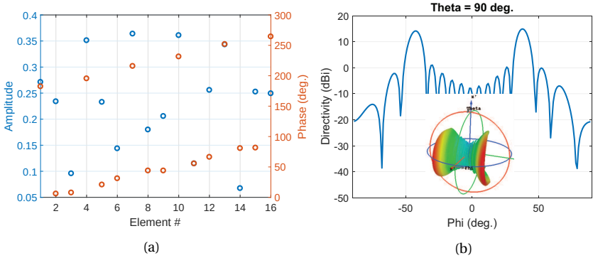
Figure 3.8: Two main-lobe 16-element array synthesis for User #20 with beams at 38 and -43 degrees: (a) amplitudes and phases, (b) radiation pattern.
