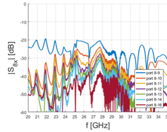
Figure 10.17: Measured mutual coupling of the microstrip line fed AC-MPA array.
