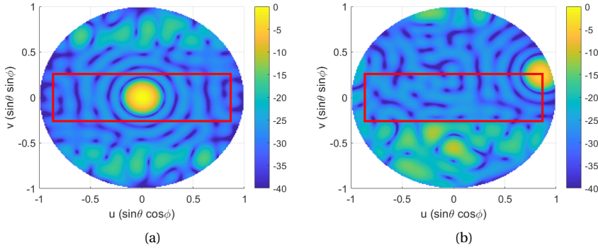
Figure 10.25: Radiation pattern at f_0 (normalized w.r.t. broadside gain, in dB) of the 64-element, fully aperiodic array with d_{\min} = 0.5\lambda : (a) broadside beam, (b) corner beam.
