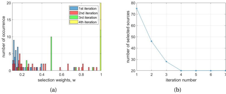
Figure 9.7: Convergence analysis of the convex optimization algorithm in Case 3 with d_g = 0.01 m: (a) Histogram of source selection weights at each iteration, (b) Number of selected sources at each iteration.
