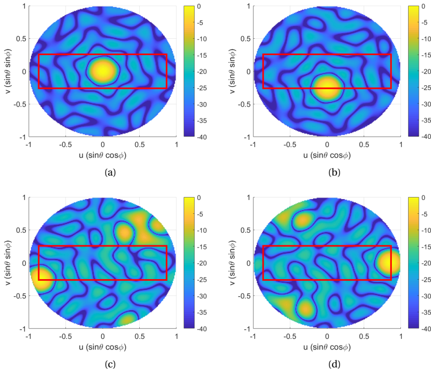
Figure 6.36: Multibeam radiation patterns (in dB, normalized w.r.t. the broadside beam) of the optimized quasi-modular 72-element array: (a) u = 0 , v = 0 , (b) u = 0 , v = -\sin \pi/12 , (c) u = -\sin \pi/3 , v = -\sin \pi/12 , (d) u = \sin \pi/3 , v = 0 .
