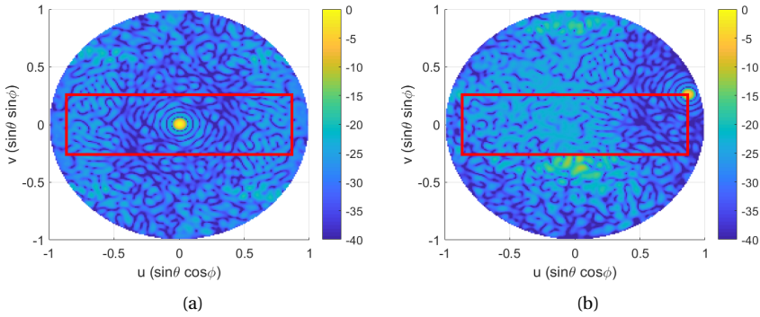
Figure 10.28: Radiation pattern at f_0 (normalized w.r.t. broadside gain, in dB) of the 256-element, fully aperiodic array with d_{\min} = 1\lambda : (a) broadside beam, (b) corner beam.
