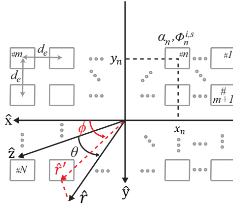
Figure 6.1: Schematic of a uniform planar array of N patch antennas. \theta is the elevation angle defined as the angle between the observation direction \hat{r} and \hat{z} . The unit vector \hat{r}' is the projection of \hat{r} onto the \hat{x}\hat{y} plane. \phi is the azimuth angle defined as the angle between \hat{r}' and \hat{x} .
