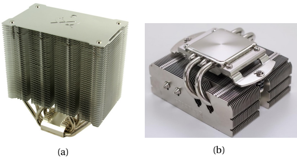
Figure 8.8: Commercial CPU heatsinks used in the paper, (a) Mugen MAX from Scythe [166], (b) NH-L9x65 from Noctua [167].
