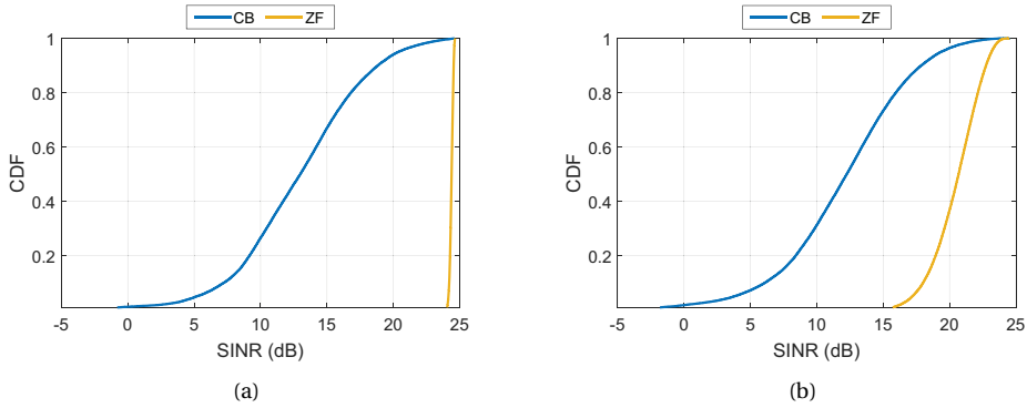
Figure 2.12: SINR results of Approach C in Use Case A: Interference-aware scheduling, imperfect CSI, non-quantized excitations, (a) max error of 0.001, (b) max error of 0.01.
