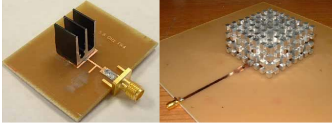
Figure 7.13: Finned and fractal heat-sink antennas [155; 156].
