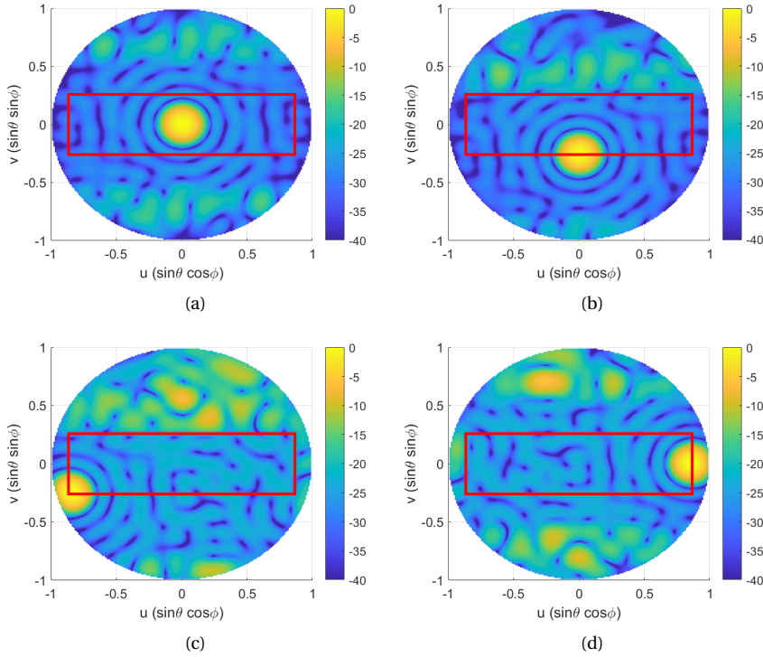
Figure 6.32: Multibeam radiation patterns (in dB, normalized w.r.t. the broadside beam) of the optimized fully-irregular 64-element array: (a) u = 0 , v = 0 , (b) u = 0 , v = -\sin \pi/12 , (c) u = -\sin \pi/3 , v = -\sin \pi/12 , (d) u = \sin \pi/3 , v = 0 .
