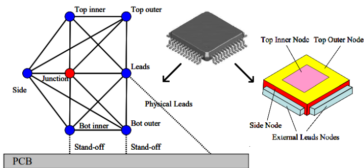
Figure 8.7: DELPHI CTM representation from [164]
