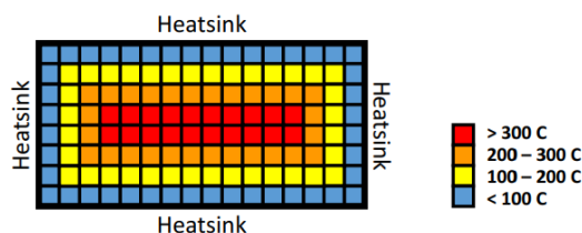
Figure 7.3: Temperature distribution across a traditional 8 \times 16 AESA [139].
