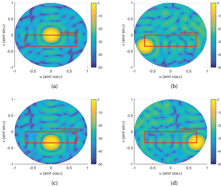
Figure 6.18: Multi-beam radiation patterns (in dB, normalized) for the test case with the optimized array with L_{\max} = 4\lambda for a beam scanned towards (a) u_{s1} = v_{s1} = 0 , (b) u_{s2} = -\sin(\pi/4) , v_{s2} = -\sin(\pi/9) , (c) u_{s3} = 0 , v_{s3} = -\sin(\pi/9) , (d) u_{s4} = \sin(\pi/4) , v_{s4} = -\sin(\pi/9) .
