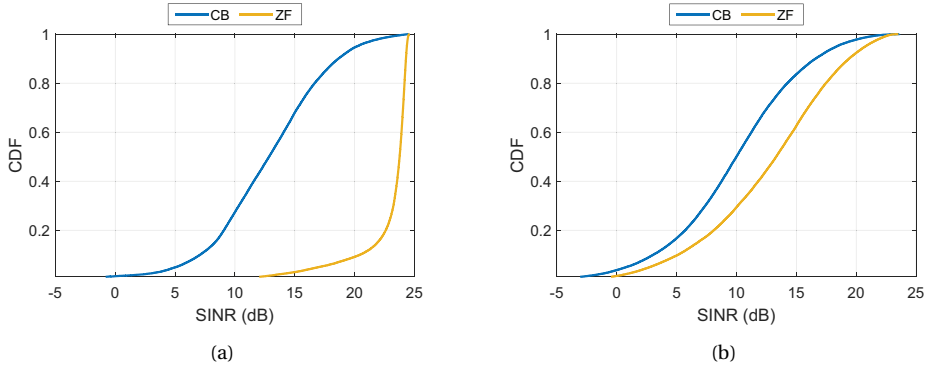
Figure 2.13: SINR results of Approach D in Use Case A: Interference-aware scheduling, perfect CSI, quantized excitations, (a) 0.5 dB amplitude step, 4-bit phase, (b) 0.5 dB amplitude step, 2-bit phase.
