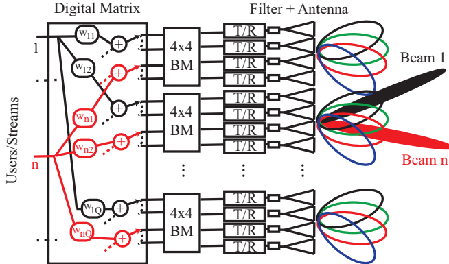
Figure 5.2: A sample use of multiport sub-arrays of 4 elements fed by 4x4 Butler Matrix to reduce DSP and hardware requirements.
