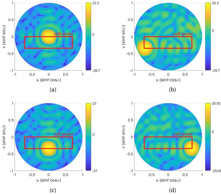
Figure 6.20: Full-wave simulation multi-beam realized gain patterns for the test case with the optimized array with L_{\max} = 4\lambda for a beam scanned towards (a) u_{s1} = v_{s1} = 0 , (b) u_{s2} = -\sin(\pi/4) , v_{s2} = -\sin(\pi/9) , (c) u_{s3} = 0 , v_{s3} = -\sin(\pi/9) , (d) u_{s4} = \sin(\pi/4) , v_{s4} = -\sin(\pi/9) .
