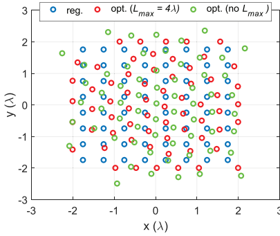
Figure 6.15: Antenna locations for the test case ( N = 64 , d_{\min} = 0.5\lambda , r_b = 0.28 , \mu = 0.08\lambda ).
