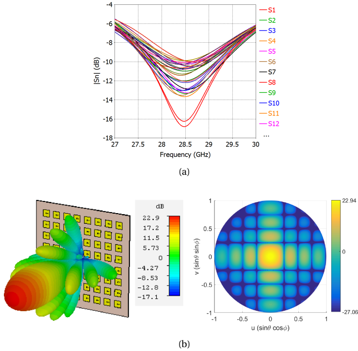
Figure 9.22: EM simulation results of the 8x8 regular square array layout with d_e = 0.5\lambda for the broadside beam including the heat spreaders, (a) active reflection coefficients, (b) realized gain at 28.5 GHz.
