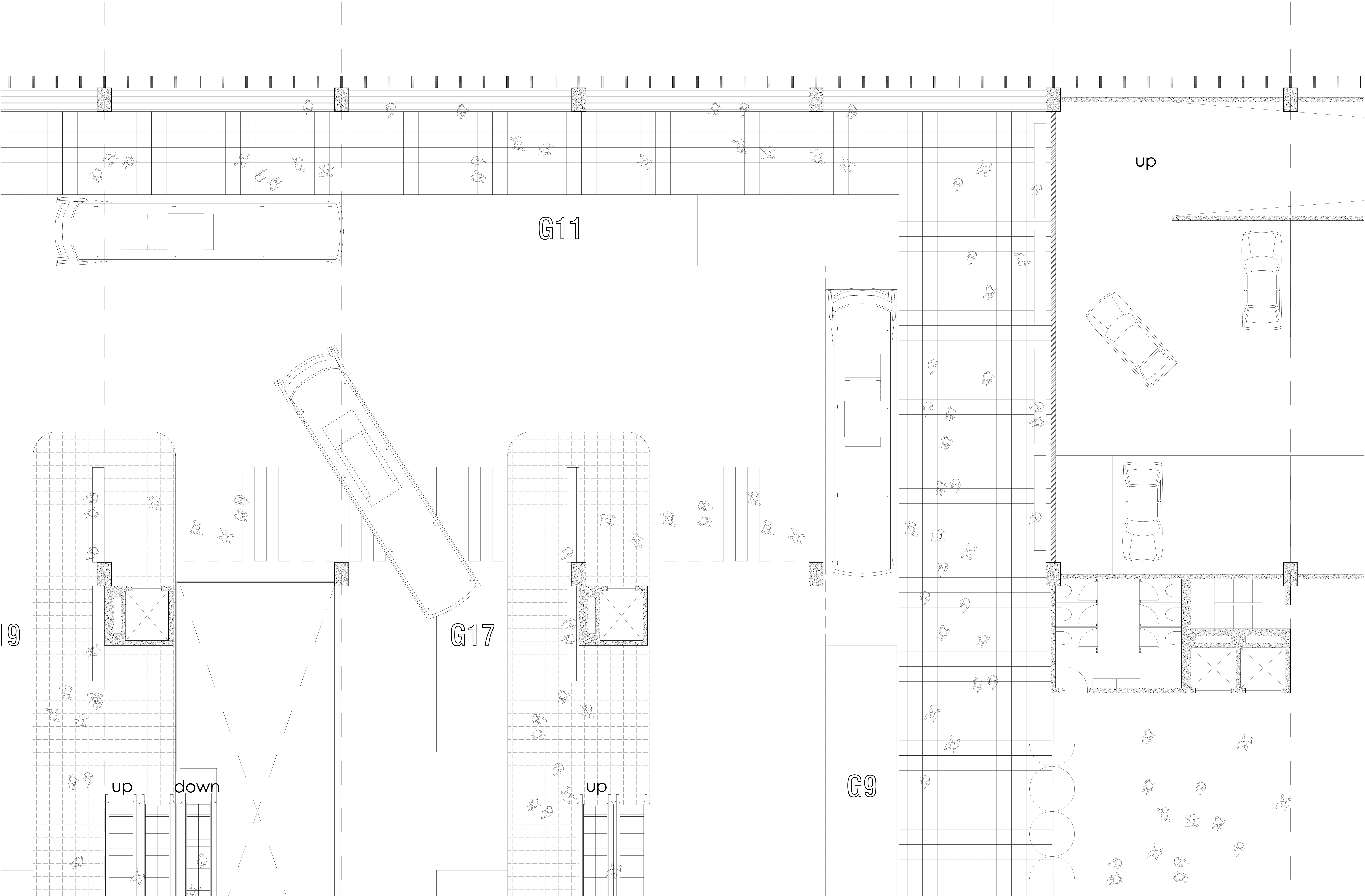
FRAGMENT: BUS TERMINAL AND PARKING LOT 1:50
