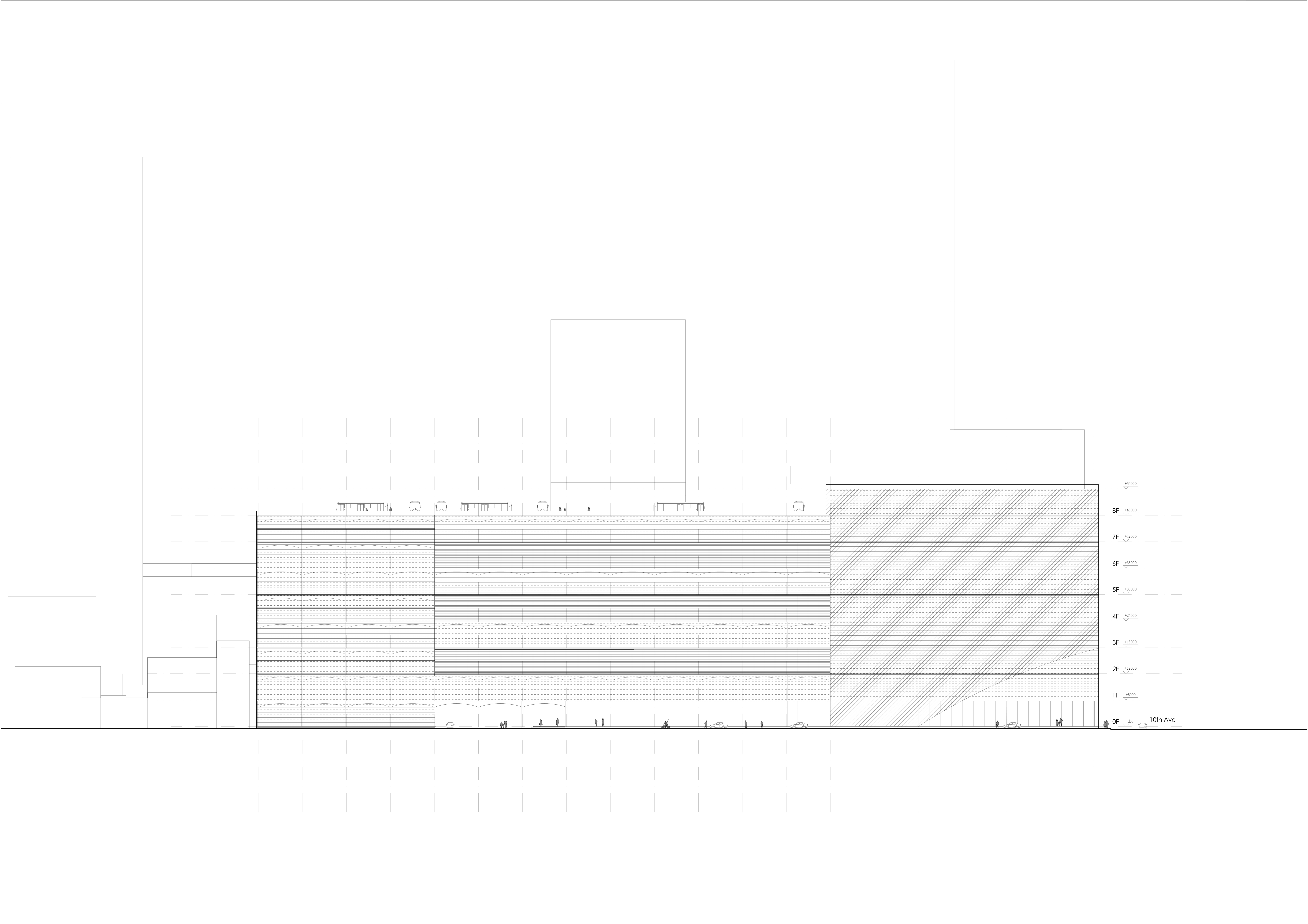
NORTH ELEVATION 1:300
