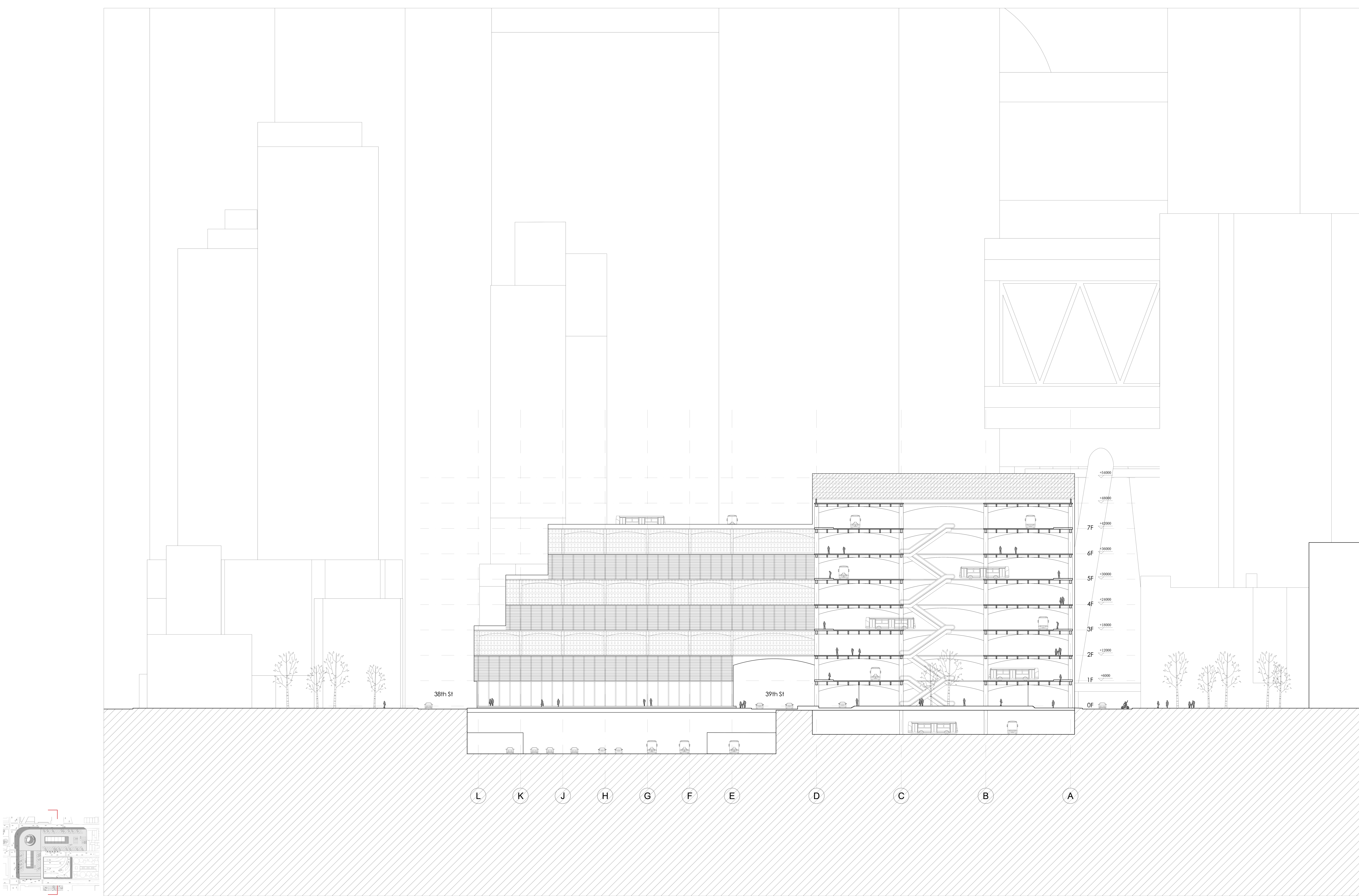
SECTION C-C 1:300
