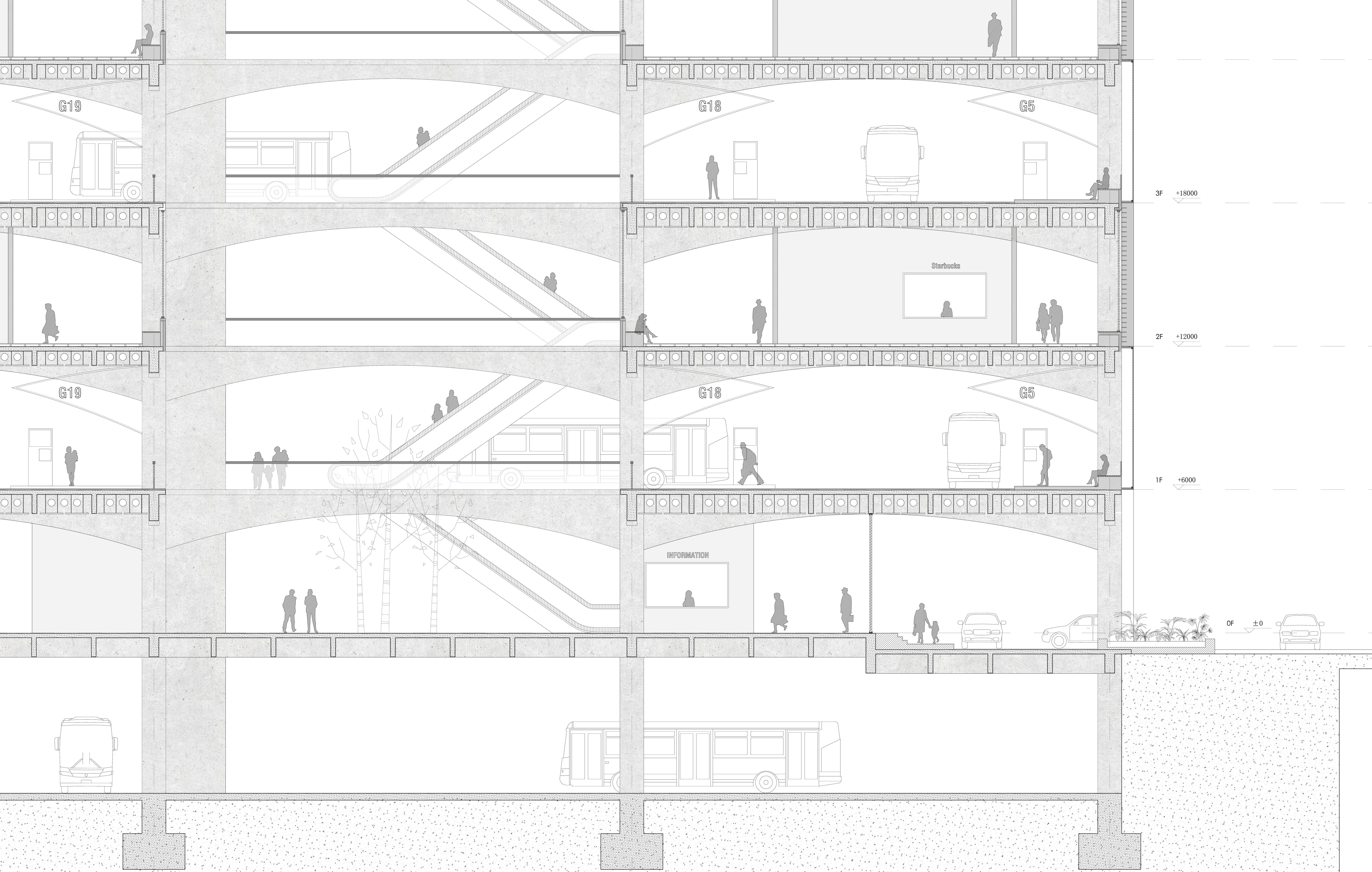
FRAGMENT: BUS TERMINAL WITH COMMERCIAL FLOOR 1:50
