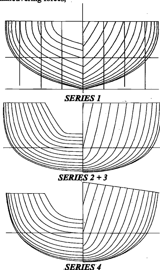
Figure 6. Body plans of the parent hulls of the DSYHS
