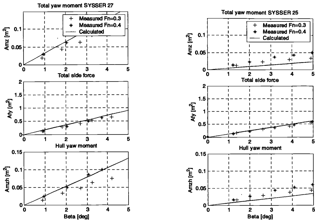
Figure 8 Side Force and Yaw Moment of DSYHS Models 15,24,25 and 27
