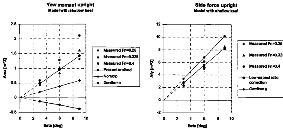
Figure 12 Side Force and Yaw Moment of a Very Large Yacht with Very Low Aspect Ratio Keel in the Upright Condition
