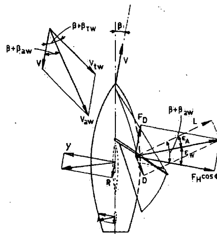
Figure 1 Definition of forces.
