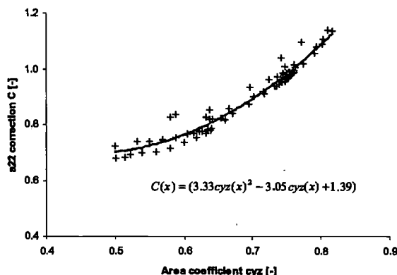
Figure 7 Sway added mass correction coefficient
