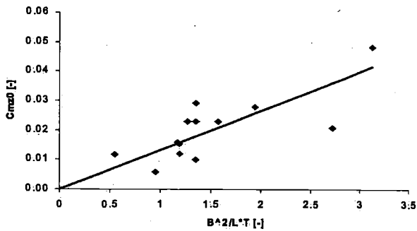
Figure 13 Offset Coefficient at 20 Degrees of Heel.
