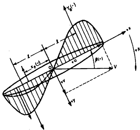
Figure 3 Force distribution on slender body in oblique potential flow. Ref [6]
