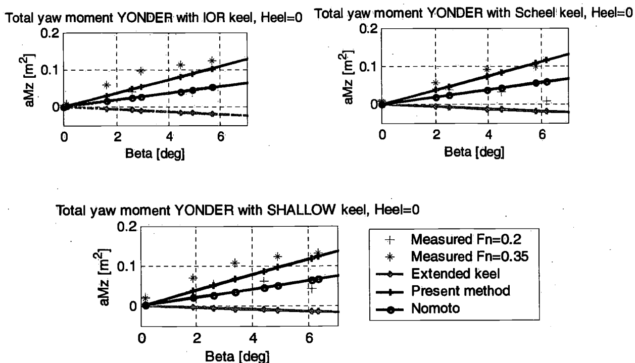
Figure 11 Measured and Calculated Yaw Moment, for the Yacht Yonder with the three different Keels:
