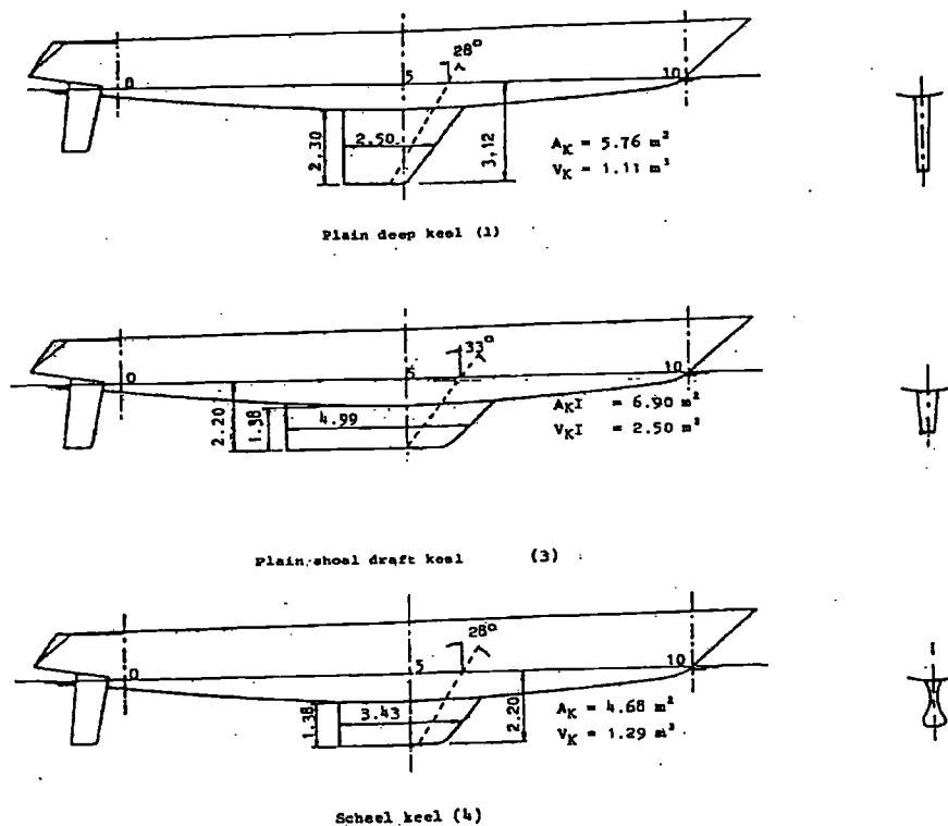
Figure 9. Layout and Main Parameters of Three Keels Tested in the DSKS L_w = 41.61 \text{ m} , B_w = 9.93 \text{ m} , b_k = 1.75 \text{ m} , C_k = 15.14 , T_c = 2.25 \text{ m}
