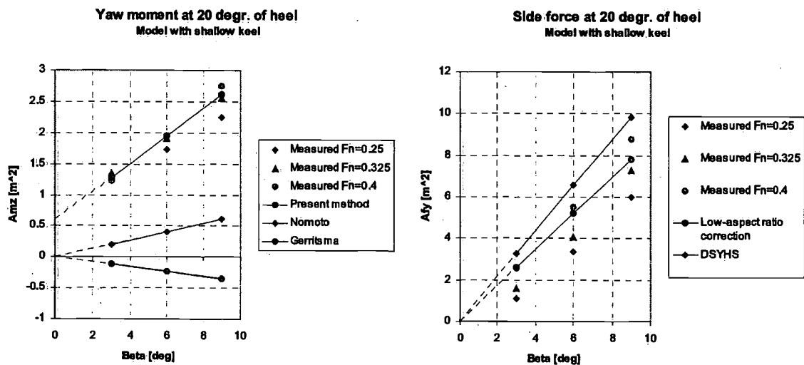
Figure 16 Side force and yaw moment of very large yacht with Very low aspect ratio keel at 20 degrees of heel
