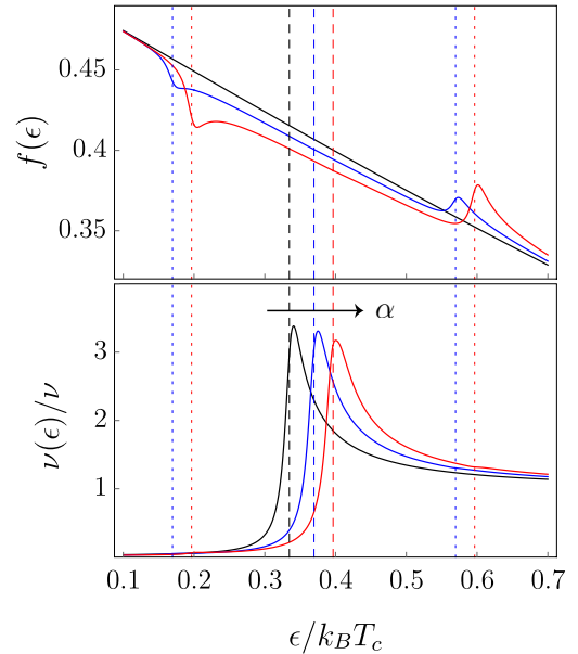
FIG. 5. Microwave-induced modification of the stationary (time-averaged) (a) quasiparticle distribution function f(\epsilon) = [1 - F(\epsilon)]/2 and (b) density of states. Black to red: \alpha/k_B T_c = 0, 0.005 , and 0.01 . The curves are plotted at T/T_c = 0.98 , \hbar\omega = 20\gamma_{\text{in}} , \gamma_{\text{in}}/k_B T_c = 0.02 , corresponding to the enhancement region in Fig. 1. The values of \Delta marked by the vertical dashed lines are obtained from the self-consistency equation. Dotted lines correspond to \Delta \pm \hbar\omega .
