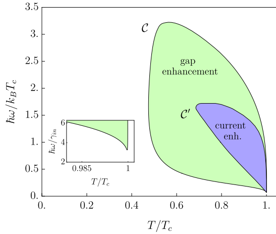
FIG. 1. Phase diagram of a superconductor under weak microwave driving ( \alpha \rightarrow 0 ) at the frequency \omega (the inelastic relaxation rate \gamma_{\text{in}}/k_B T_c = 0.02 ). Gap enhancement is observed inside the curve C . The region of the critical current enhancement is bounded by the curve C' . Inset: zoom of the gap enhancement region near T_c , showing the minimal frequency \omega_{\text{min,min}} \approx 3.23 \gamma_{\text{in}}/\hbar .
