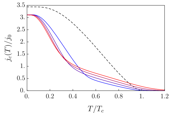
FIG. 7. Critical current as a function of temperature at fixed radiation intensity \alpha = 0.1k_B T_c and varying frequency. Black dashed line: without irradiation; color lines: frequency 0.1k_B T_c/\hbar to 0.4k_B T_c/\hbar from blue to red; \gamma_{\text{in}}/k_B T_c = 0.02 .
