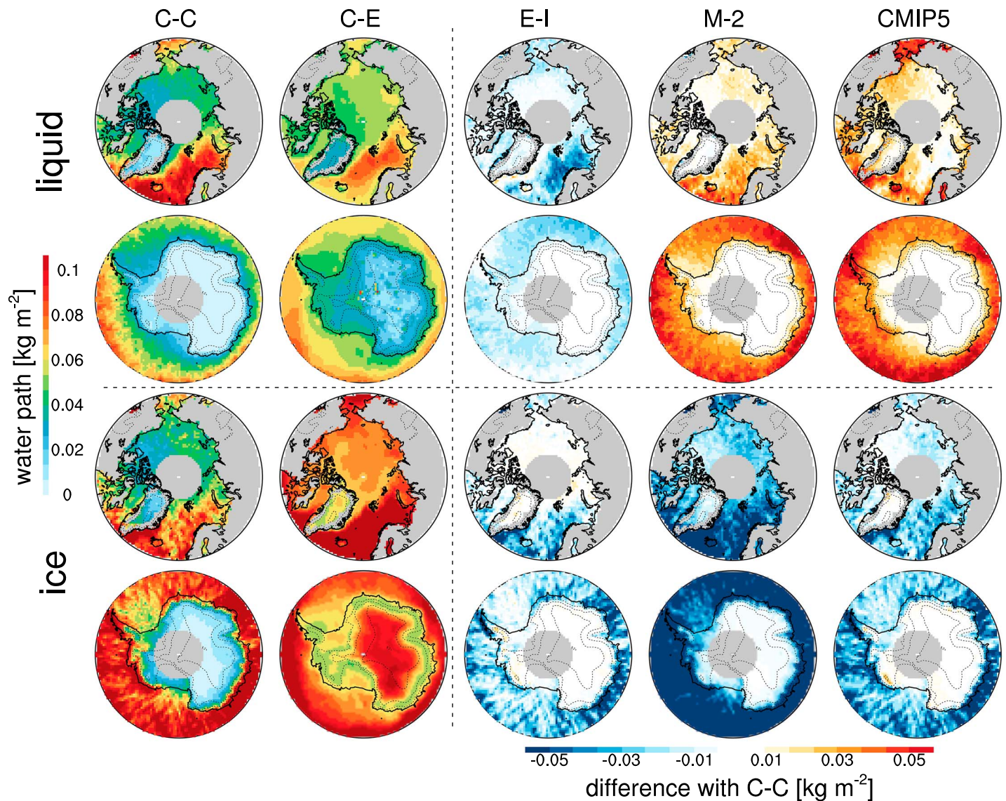
Figure 1. (first and second rows) Cloud liquid and (third and fourth rows) ice for the Arctic Ocean and Greenland (Arctic land regions are shown in grey and are not considered in this study) and the Southern Ocean and Antarctica according to the (first column) CloudSat-CALIPSO (C-C) and (second column) CERES-EBAF (C-E). The ocean regions include both ocean and sea ice-covered pixels. The simulated cloud LWP and IWP in (third column) ERA-Interim (E-I), (fourth column) MERRA-2 (M-2), and (fifth column) CMIP5 (avg) are plotted as absolute differences with C-C.
