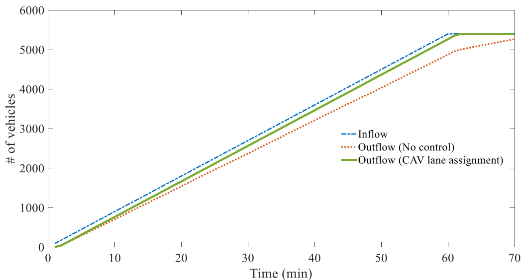
Figure 7.6: Cumulative curves at the diverge bottleneck
