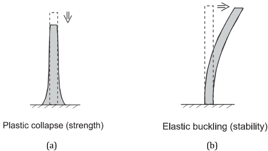
Fig. 12. Wall failure mode during printing process (Suiker, 2018) (a) plastic collapse, which is dominant by material strength (b) elastic buckling, which is dominant by material stiffness.
