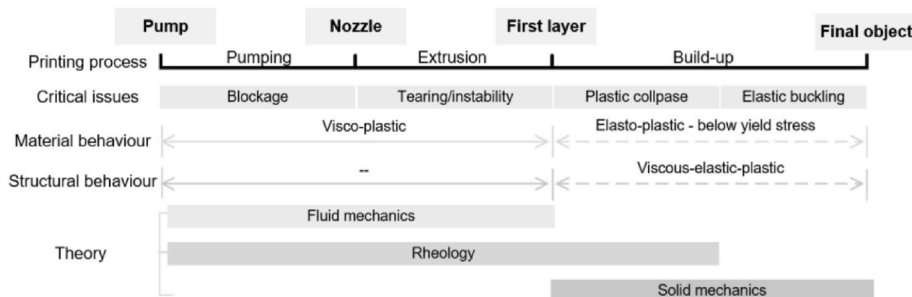
Fig. 2. A schematic diagram of 3DCP at different stages (Chang et al., 2021).
