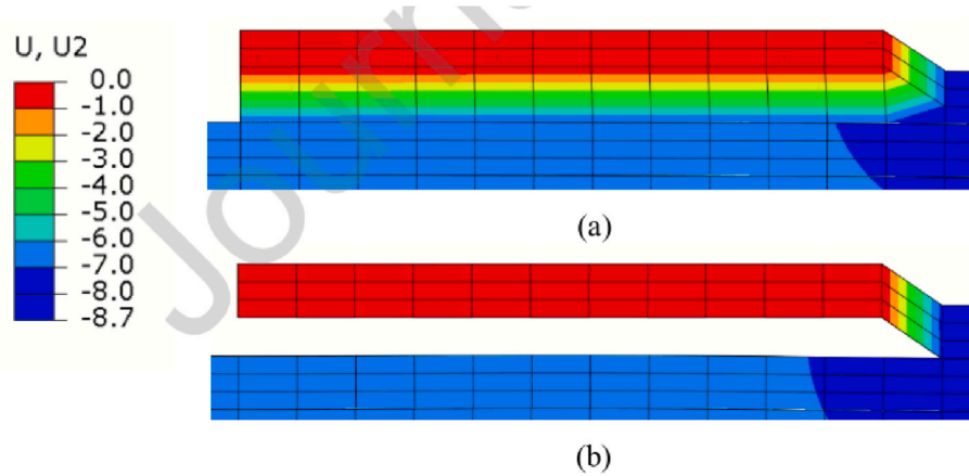
Fig. 20. Different interactions in ABAQUS: (a) tie constraints (b) contact-based interactions (Ooms et al., 2021).
