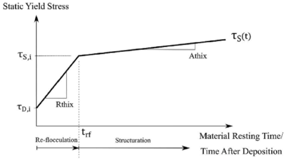
Fig. 11. The development of static yield stress as a function of the concrete age with the consideration of re-flocculation and structuration, the different stages can be mathematically described by Eqs. (2)–(4) (Kruger et al., 2019e).
