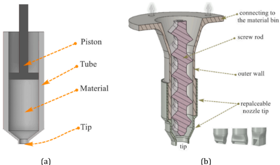
Fig. 4. Two commonly used extruder types in 3DCP (Cao et al., 2022) (a) a piston extruder; (b) a screw-type extruder.
