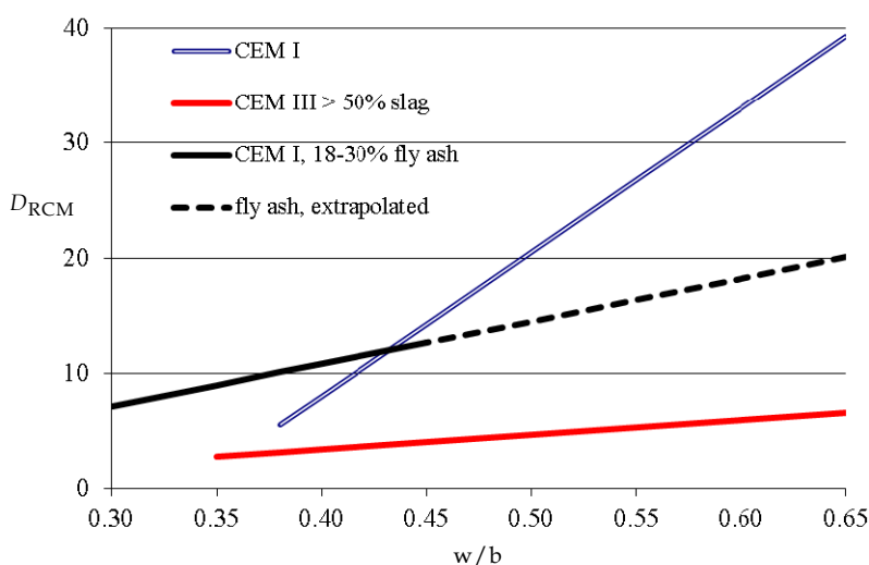
Figure 2: Correlation between w/b (-) and D_{\text{RCM}} at about 28 days; D_{\text{RCM}} values \cdot 10^{-12} \text{ m}^2/\text{s}
