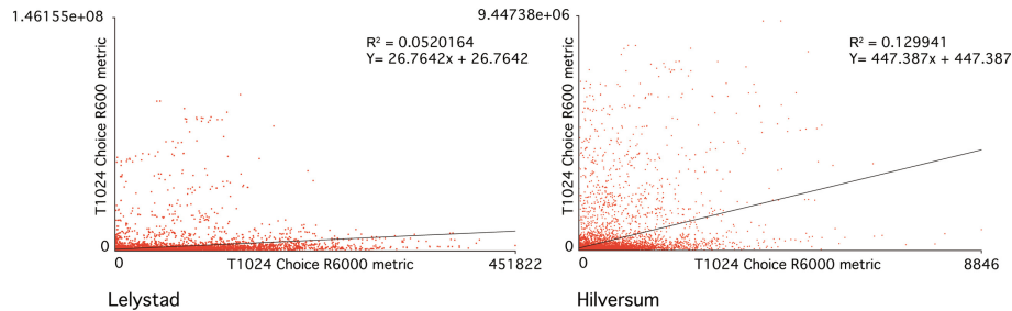
Fig. 2.48 Scatterplots for Lelystad (left) and Hilversum (right)
