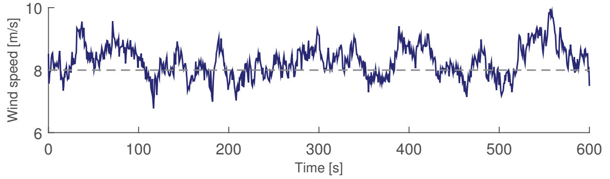
Fig. 10. Wind speed time series with 8.0 m/s mean value and 12% turbulence intensity used for the time-domain simulations.
