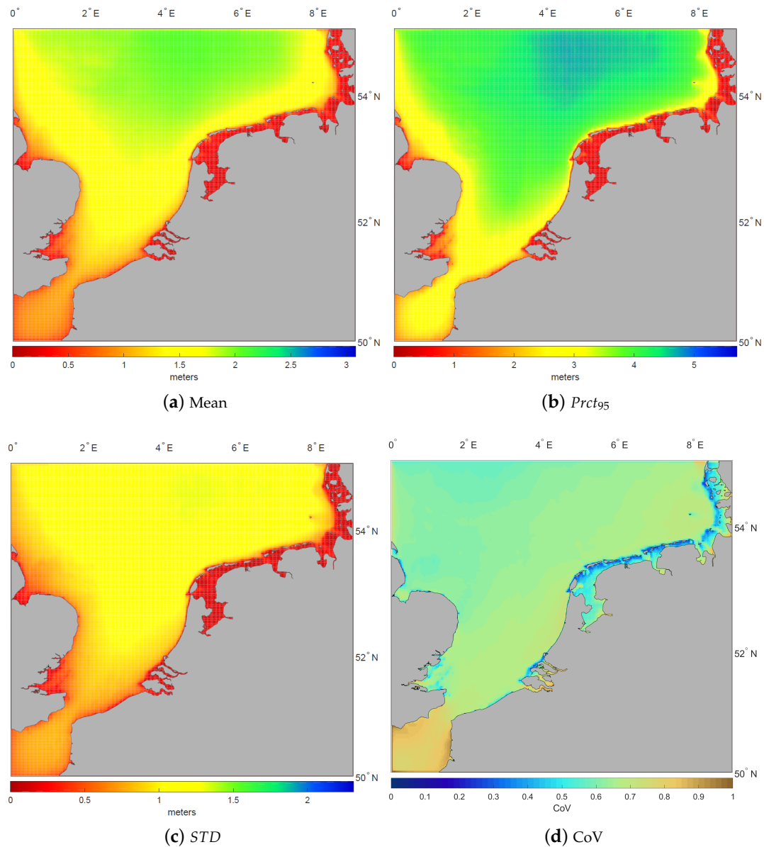
Figure 11. H_{m0} statistics.
