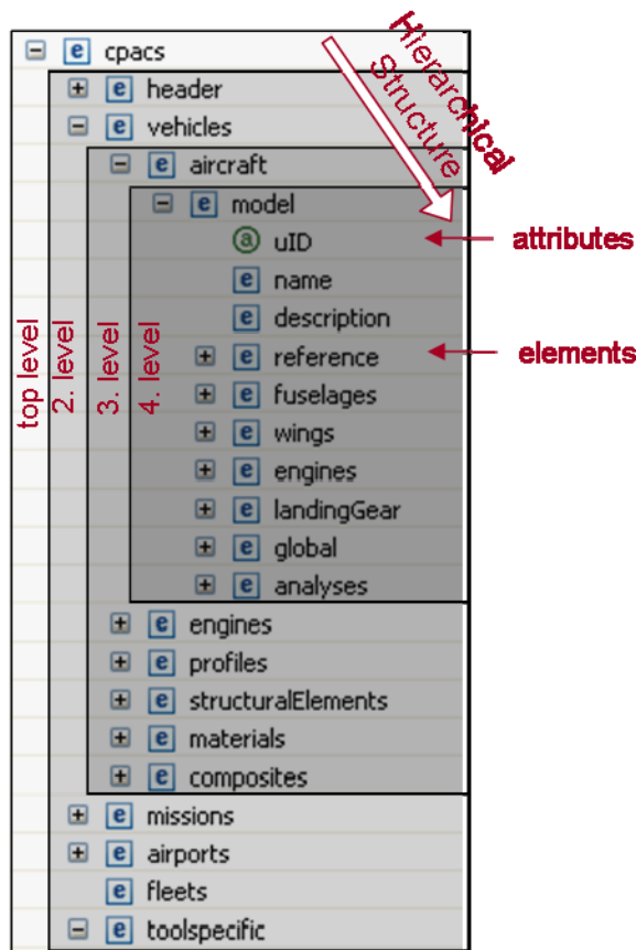
FIGURE 3. CPACS Structure
