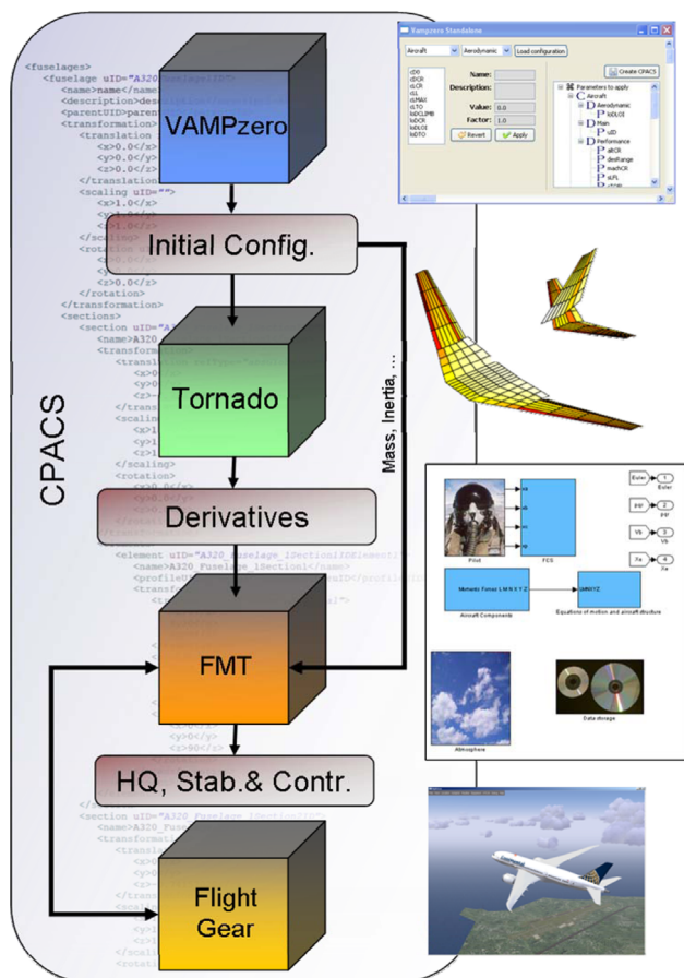
FIGURE 5. Example Framework with Tornado as Aerodynamic Method
