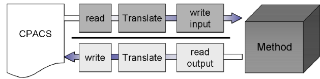
FIGURE 4. CPACS Wrapper
