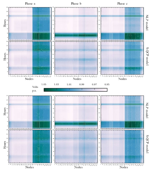
Figure 8. 123 node test feeder voltage magnitudes for the min. scenario, with PV reactive compensation (first two rows) and without PV reactive compensation (last two rows). Source: The authors.
