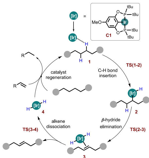
Scheme 2. Catalytic Cycle for the ( t Bu 4 POCOP)-Ir Catalyzed Transfer Dehydrogenation of PE
