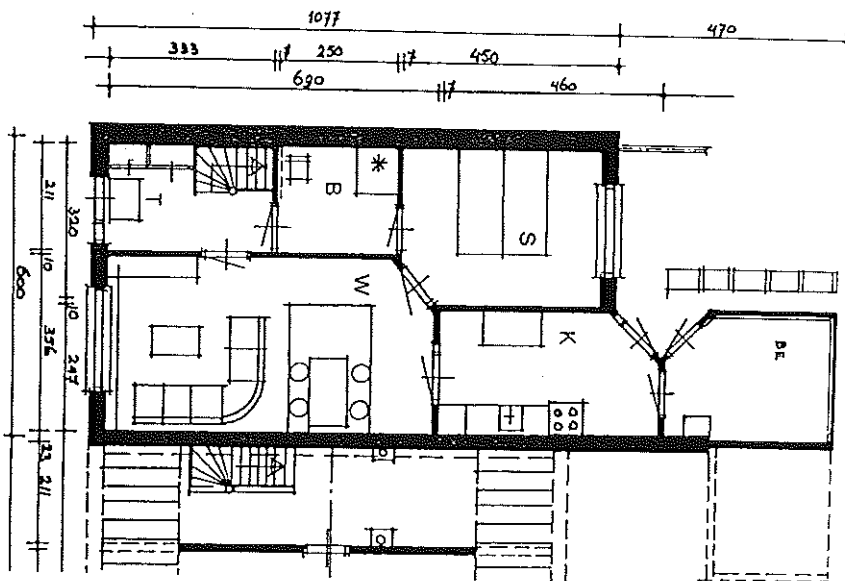
Fig. 2d: Floor plans of one-family homes in Oosterhout - the same design in adapted state, intended for use by disabled person confined to wheelchair, yet having normal arm and hand functions and capable of performing own domestic duties. Legend: T = entrance hallway, W = living room, S = bedroom, K = kitchen, B = bathroom/toilet, Be = storage.
