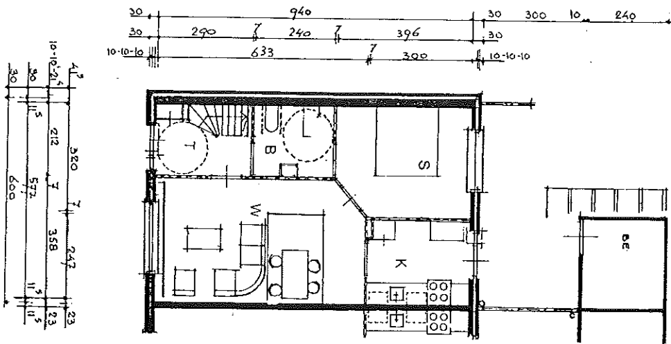
Fig. 2c: Floor plans of one-family homes in Oosterhout - adaptable design, second series of 24 homes. Legend: T = entrance hallway, W = living room, S = bedroom, K = kitchen, B = bathroom/toilet, Be = storage.
