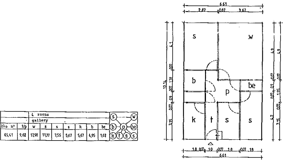
Fig. 4a Layout variant type 5 ('Era-flat'), according to minimum measurements of four systems of standards: Model Building Ordinance, 22nd supplement (MBV22).
