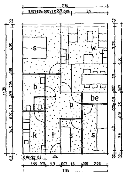
Fig. 4c Layout variant type 5 ('Era-flat'), according to minimum measurements of four systems of standards: Requirements for Building Adaptable Housing (NWR).
