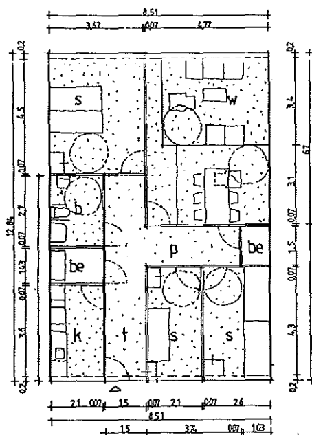
Fig. 4d Layout variant type 5 ('Era-flat'), according to minimum measurements of four systems of standards: "Call for Admittance" (GT).
