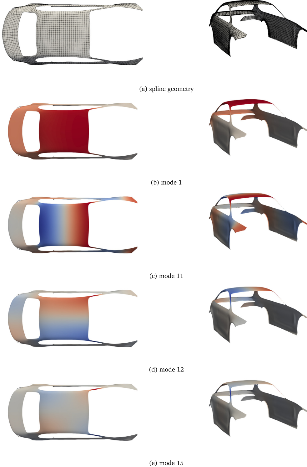
Fig. 14. The figure in the top row shows a part of a BMW car — the model is a Blender® demofile, a coarse quadrilateral mesh for it was generated using Rhinoceros® and the spline geometry was constructed on that mesh using our unstructured splines. The bottom rows show select eigenmodes corresponding to the Laplace–Beltrami eigenvalue problem (Section 5.5) solved on this geometry. The mesh contains 4482 faces and 5330 dofs.
