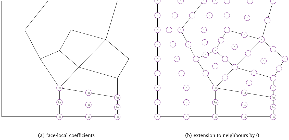
Fig. 4. Here we take a submesh of the one from Fig. 2(a) to illustrate how the extraction coefficients will be graphically denoted. Given a face \sigma \in \mathcal{T} and \phi such that \phi \cap \sigma = \phi , B_\phi^* will be defined graphically by specifying its Bernstein–Bézier coefficients on \sigma ; see figure (a). This description will be extended to neighbouring faces of \mathcal{T} with zero coefficients denoted here with a \cdot in figure (b). See Section 3.2 for further elaboration.
