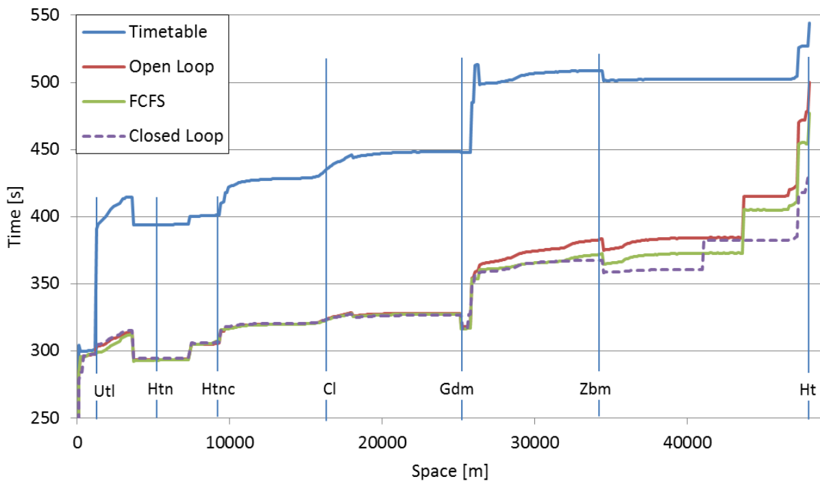
Figure 8. Average time deviations from scheduled train paths
