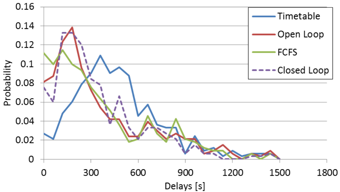
Figure 10. Statistic distribution of arrival delays at the final station.
