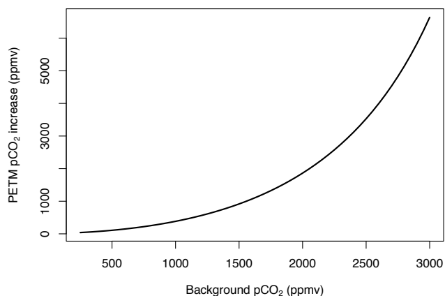
Figure B1. Figure showing p_{\text{PETM}} and change in PETM p\text{CO}_2 ( Dp_{\text{PETM}} ) across a range of assumed background p\text{CO}_2 conditions from 250 to 3000 ppmv.
