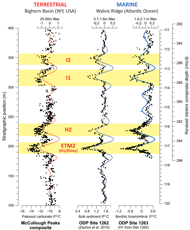
Figure 3. The McCullough Peaks paleosol carbonate carbon isotope stratigraphy compared in-depth domain to the bulk sediment and benthic foraminiferal ( Nuttallides truempyi ) carbon isotope stratigraphies at, respectively, ODP Site 1262 (left y axis on right side; Zachos et al., 2010) and 1263 (right y axis on right side; Stap et al., 2010a; this study) at Walvis Ridge in the southern Atlantic Ocean. Filters denote the ~100 kyr eccentricity band in the three records. Note that linear stretching of depth scales is sufficient to construct the figure, indicating the constant average sedimentation rates on longer timescales in both realms. On smaller timescales, large sedimentation rate differences occur that in the marine realm relate to carbonate dissolution during and carbonate overshoot after the hyperthermal events.
