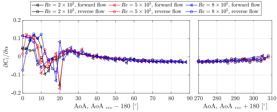
FIGURE 7 | C_l slope in forward flow and reverse flow conditions at three Re values.
