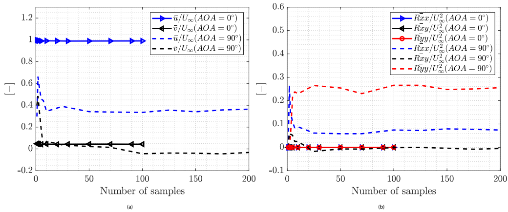
FIGURE C1 | Evolution of the statistical (a) average velocity and (b) Reynolds stresses at Re = 5 \times 10^5 at AoA = 0^\circ and 90^\circ .
