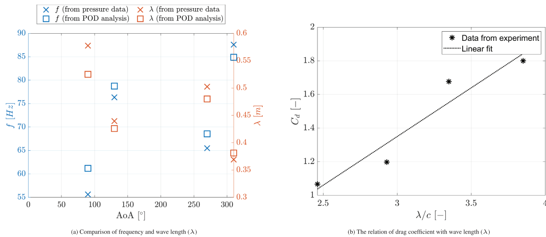
FIGURE 20 | Comparison of frequency and wavelength ( \lambda ) from experiment measurement and from POD analysis (left) and the relation of drag coefficient with wavelength ( \lambda ). On the right figure, the data from experiments from left to right are the case of AoA 310^\circ , 130^\circ , 270^\circ , and 90^\circ .
