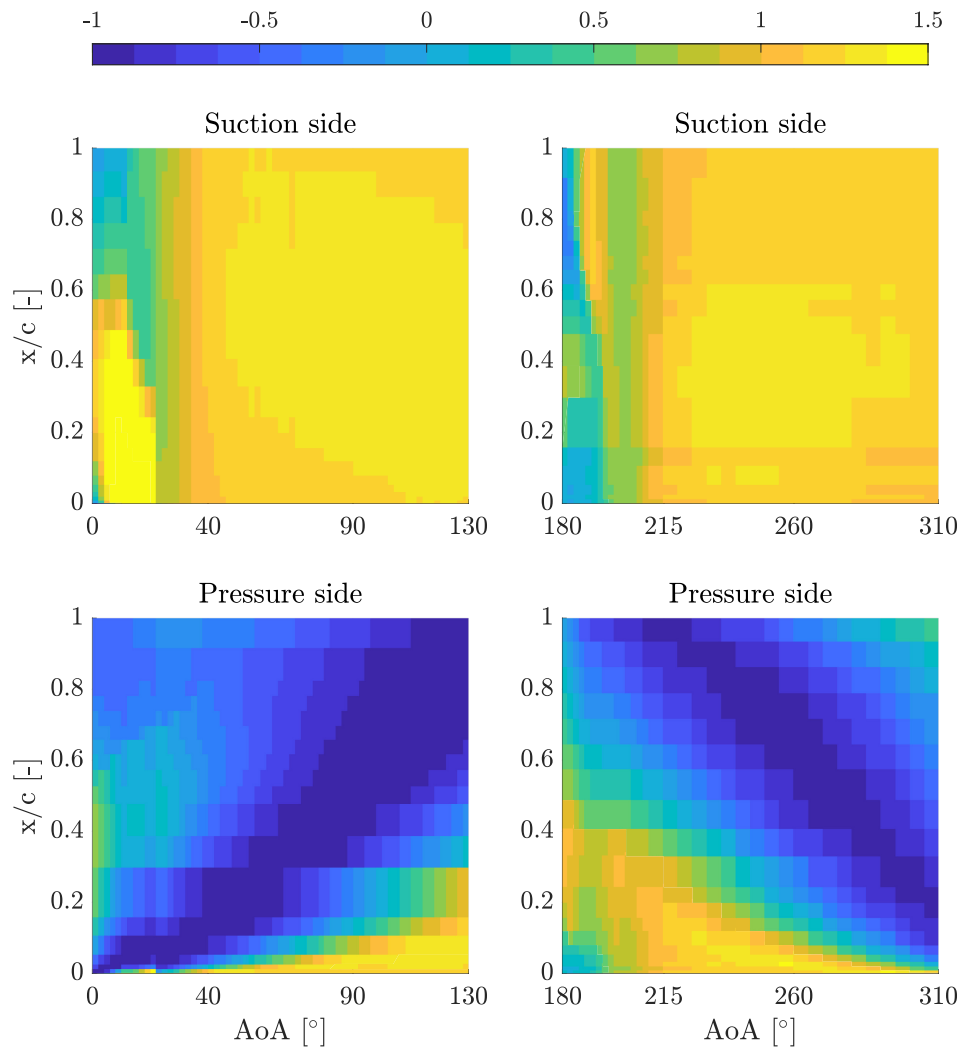
FIGURE 12 | Average of pressure coefficient -C_p for all AoA values tested at Re = 5 \times 10^5 . Note that the suction side is the different side for AoA larger than 180^\circ .
