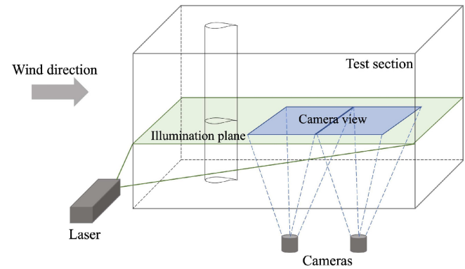
FIGURE 2 | PIV setup.
