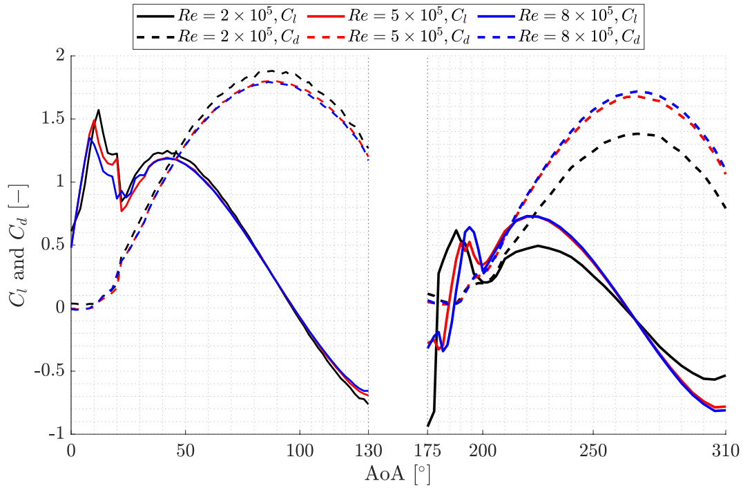
FIGURE 3 | Aerodynamic performance of DU91-W2-150 at three Re values.
