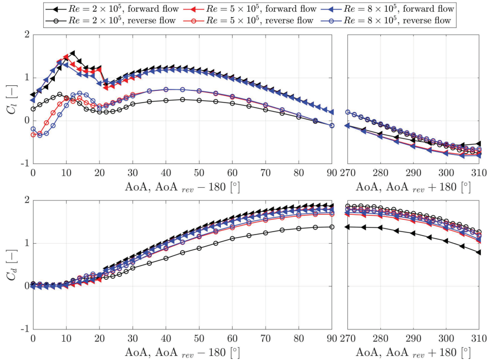
FIGURE 5 | Aerodynamic performance in forward flow and reverse flow conditions at three Re values.
