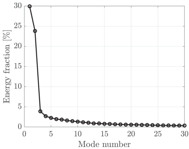
FIGURE 17 | Energy fraction for the first 30 modes at 90^\circ in Re 5 \times 10^5 .
