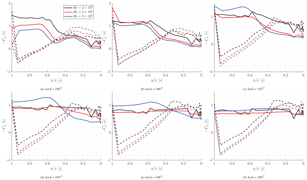
FIGURE 9 | Pressure coefficient C_p near the negative stall region for all the measured Re values. The x direction was flipped in the plot which shows the geometric leading edge first as it serves as the aerodynamic leading edge. The pressure side are shown as dashed in order for clarification.
