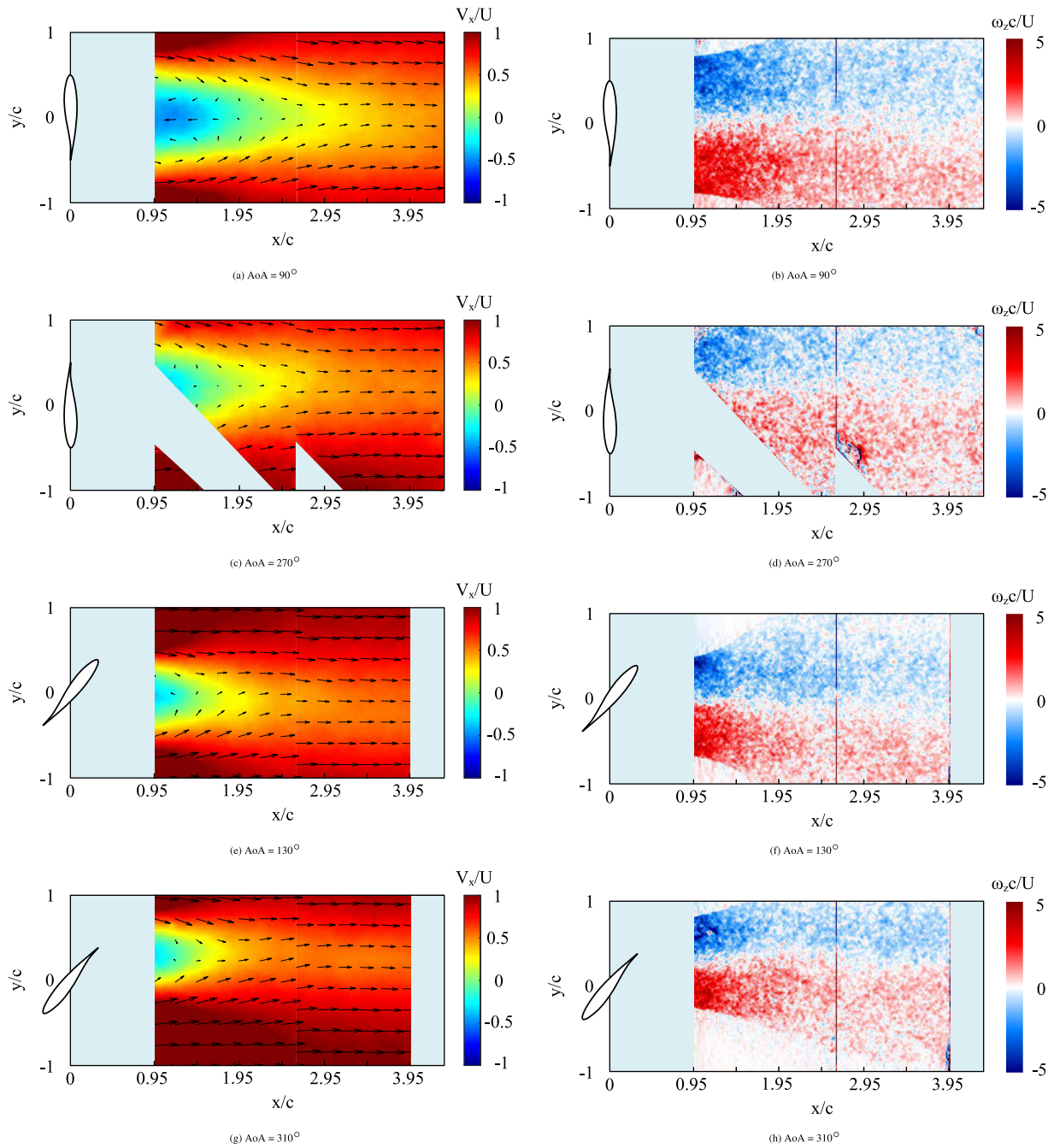
FIGURE 13 | Mean flow field (left column) and vorticity field (right column) at AoA = 90^\circ, 270^\circ, 130^\circ , and 310^\circ , Re = 5 \times 10^5 .
