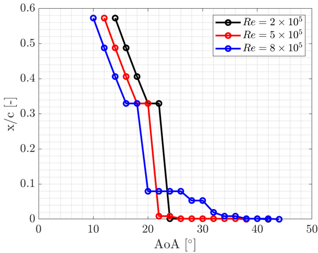
FIGURE 10 | Separation locations on the airfoil surface on the suction side for different Re values.
