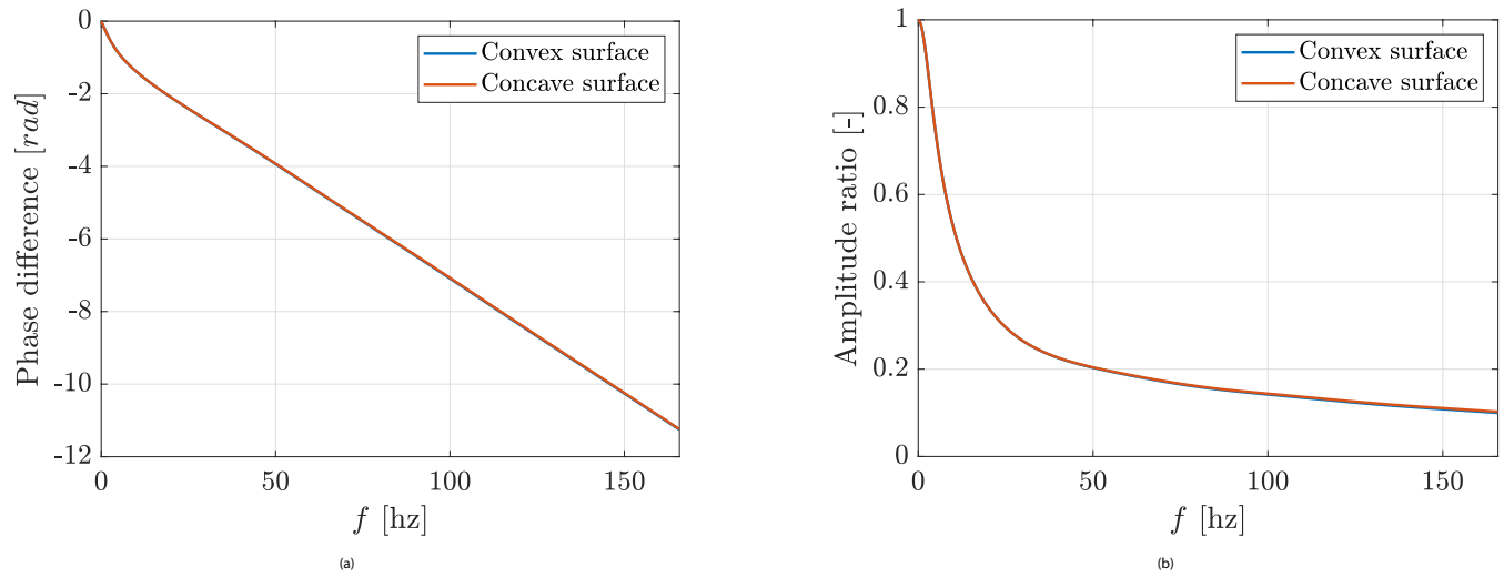
FIGURE A1 | Transfer function in the frequency domain for dynamic response correction of the pressure measurement system.
