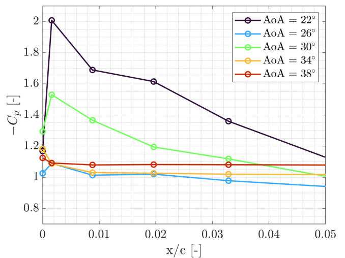
FIGURE 11 | Leading edge surface pressure for AoA from 20^\circ to 38^\circ at Re = 8 \times 10^5 .
