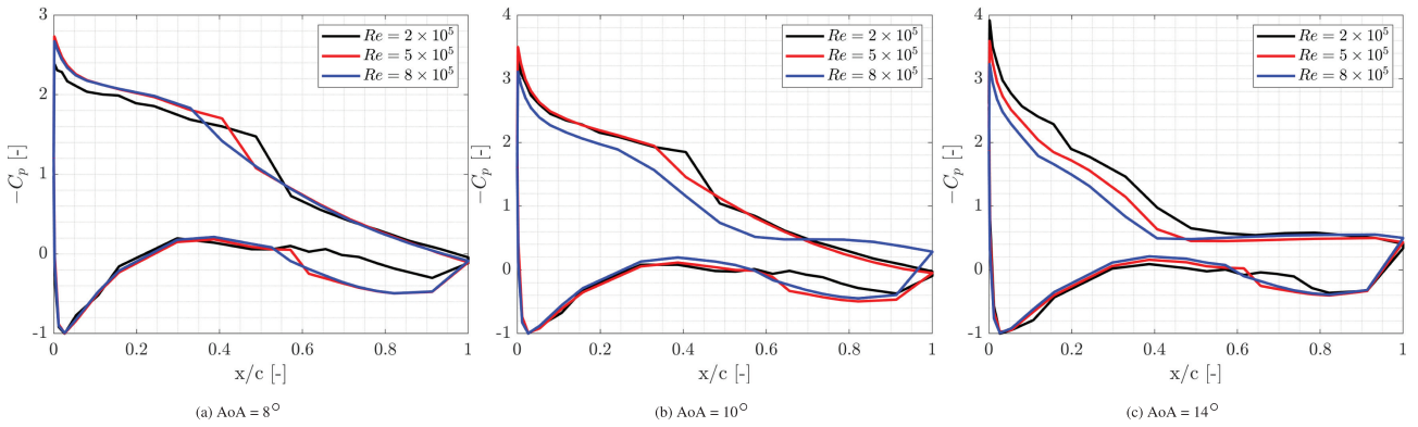
FIGURE 8 | Pressure coefficient C_p near the possible stall region for all the measured Re values.
