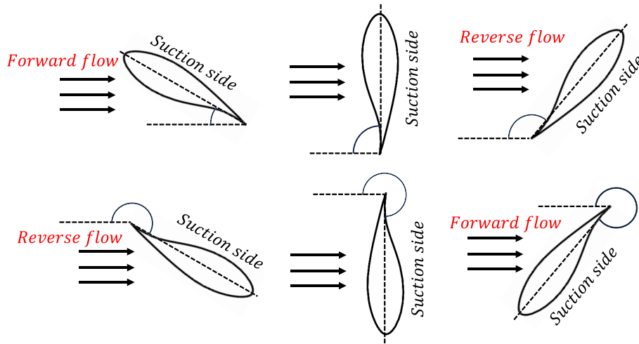
FIGURE 4 | Schematic plot of different AoA values tested in the campaign. The wind comes from left to right. The corresponding AoA is 30°, 90°, and 130° for the first row and 210°, 270°, and 310° for the second row. When the geometric trailing edge is facing the front wind, reverse flow occurs.
