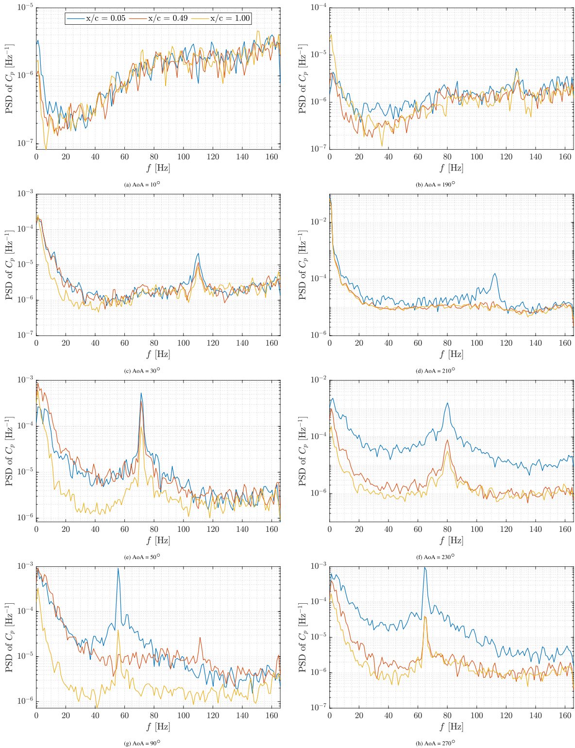
FIGURE 18 | FFT of C_p at airfoil suction surface at Re = 5 \times 10^5 .
