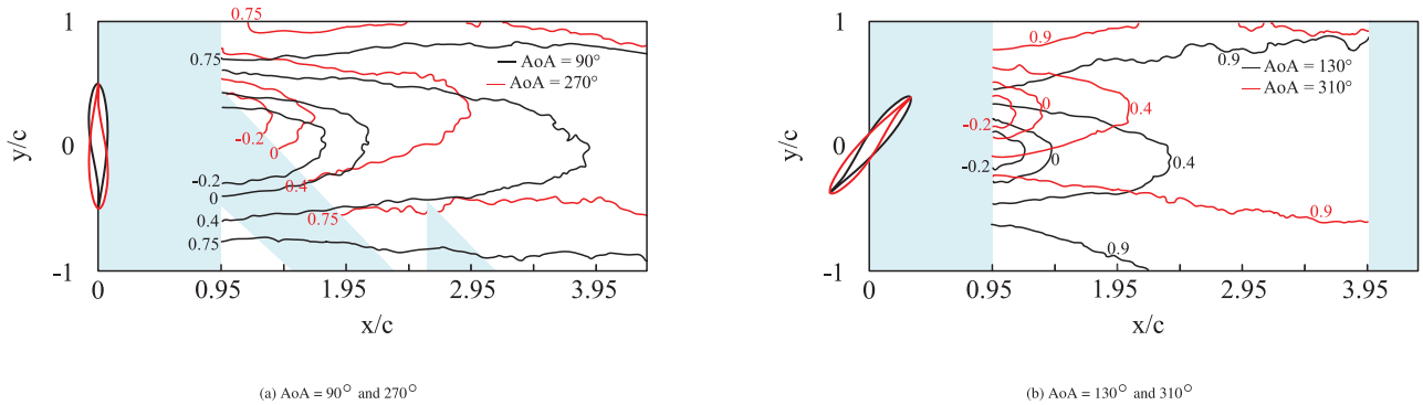
FIGURE 14 | Wake contour lines of V_x/U = -0.2, 0, 0.4 and 0.75(0.9) for several AoA values at Re = 5 \times 10^5 . Note that the contour line V_x/U = 0.75 was plotted for 90^\circ and 270^\circ while V_x/U = 0.9 was plotted for 130^\circ and 310^\circ .
