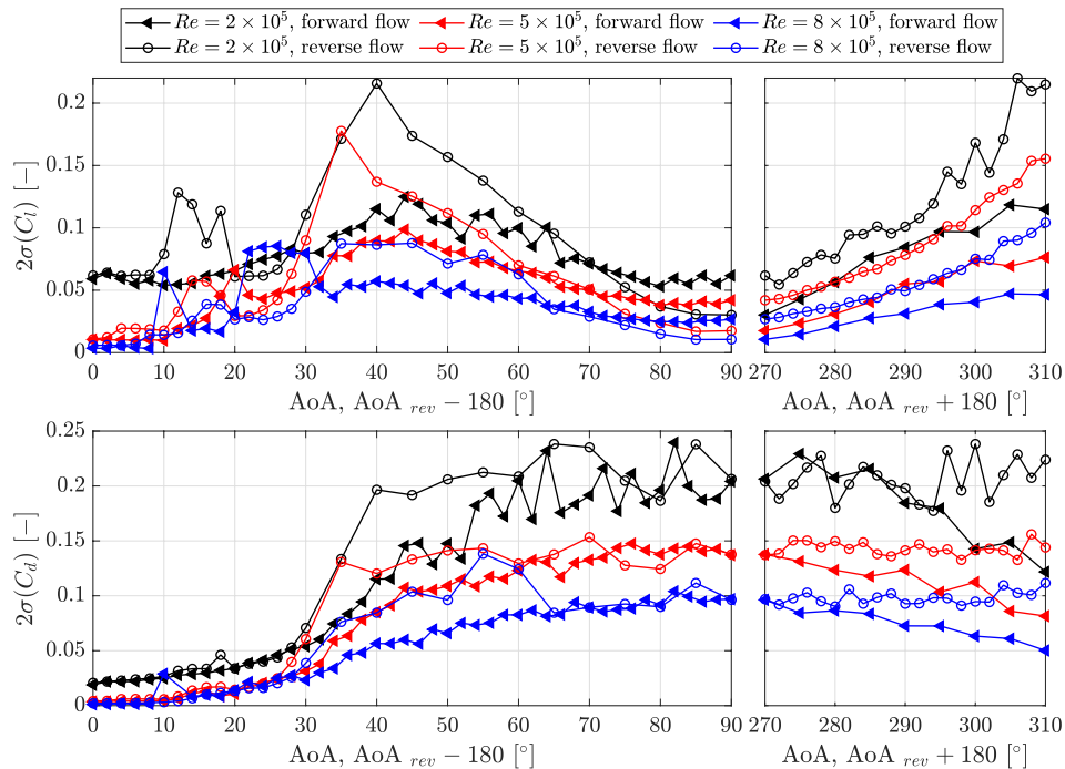
FIGURE 15 | Fluctuations (two times the standard deviation 2\sigma ) of unsteady C_l and C_d for different Re values in the forward flow and reverse flow conditions.
