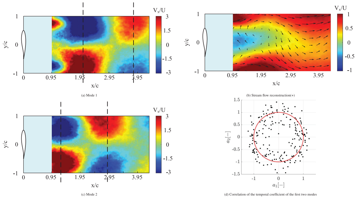
FIGURE 16 | POD mode analysis at \text{AoA} = 90^\circ , Re = 5 \times 10^5 . (a, c) First two modes. (b) Corresponding wake reconstruction based on the first two modes. (d) Correlation of the temporal coefficient of the first two modes.
