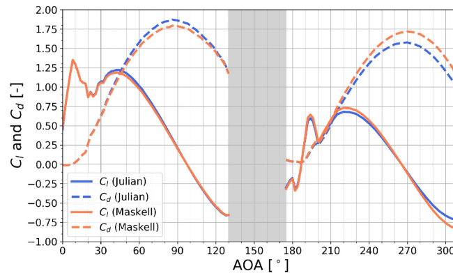
FIGURE B1 | Comparison of two blockage correction method for Re = 8 \times 10^5 (Gray area represents the AoA values that out of range of measurement).
