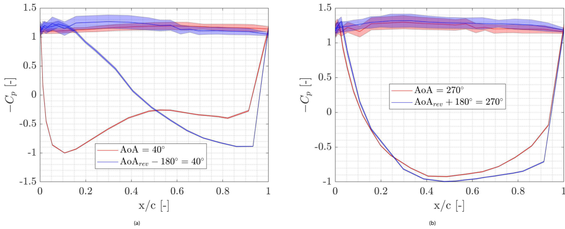
FIGURE 6 | Surface pressure comparison between forward flow and the corresponding reverse flow angle at Re = 5 \times 10^5 . Shaded area represents the standard deviation.
