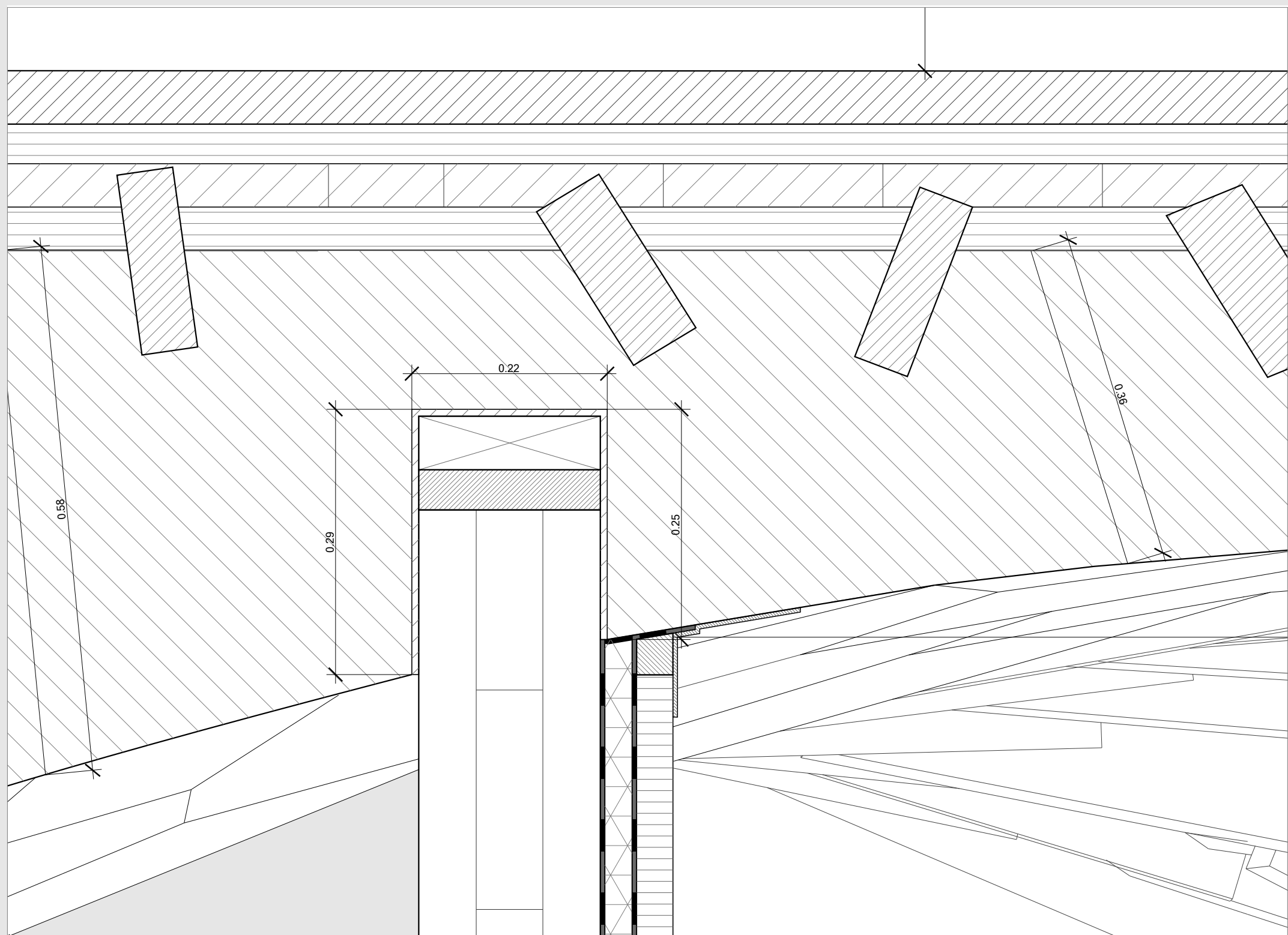
e - 1:50 Detail Section
