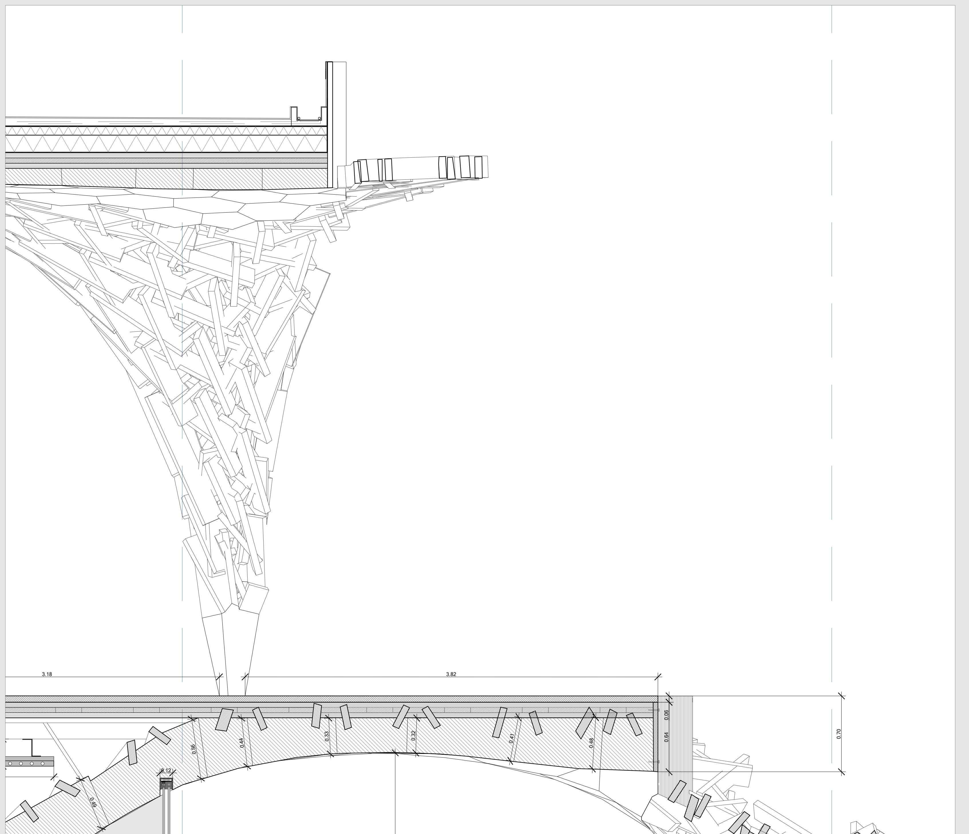
a - 1:20 Detail Section
