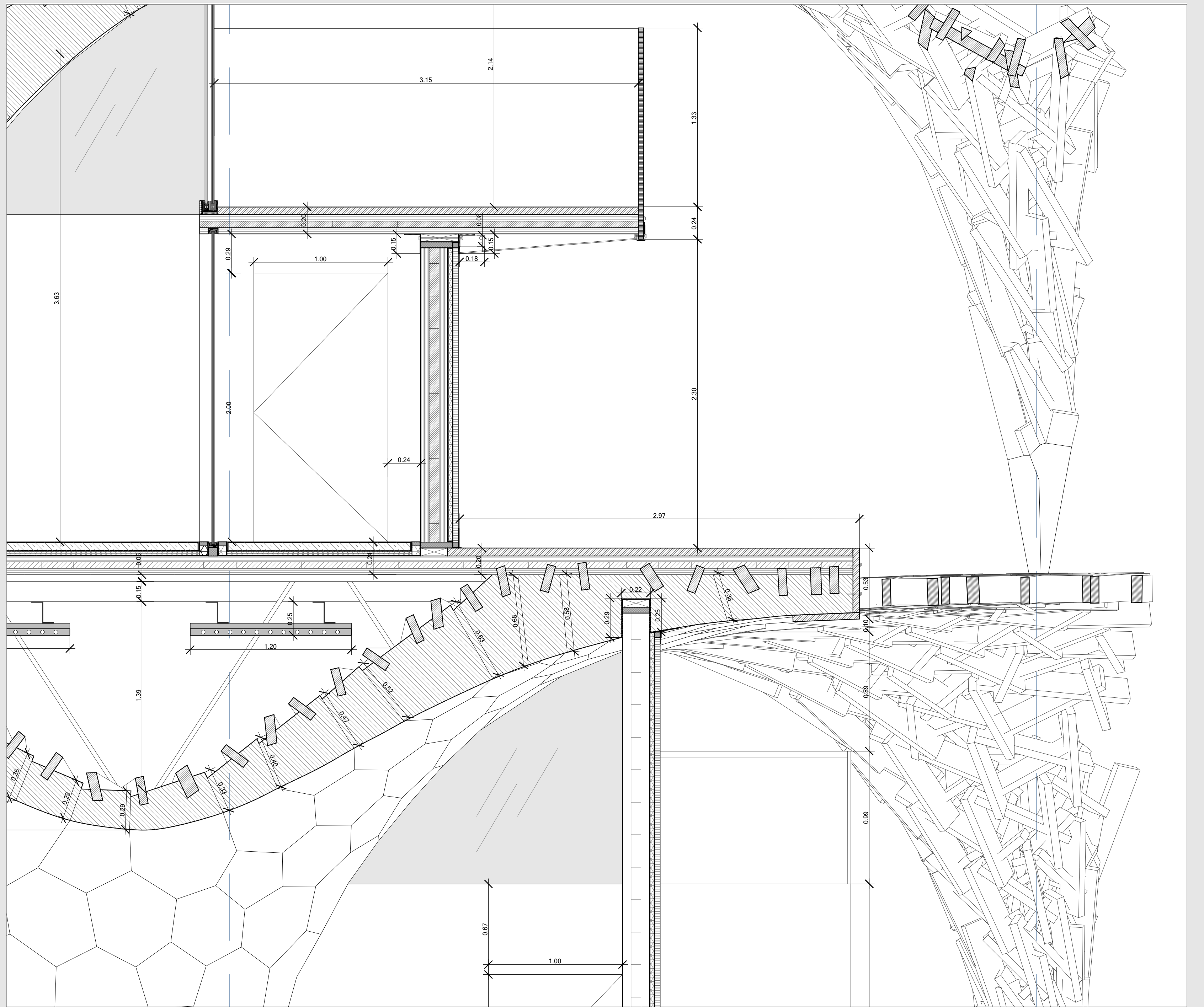
b - 1:20 Detail Section
