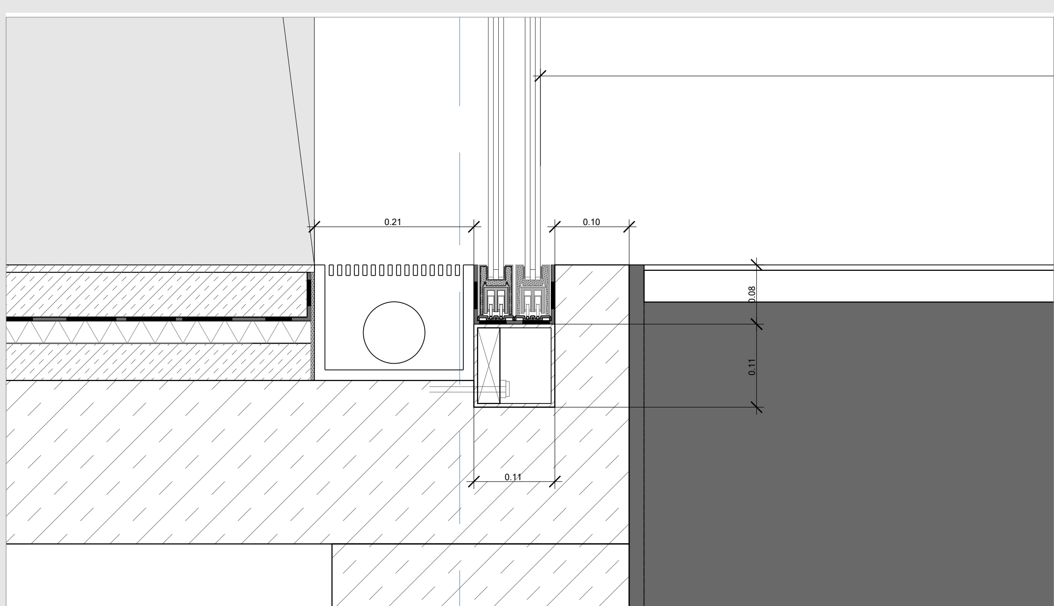
g - 1:50 Detail Section
