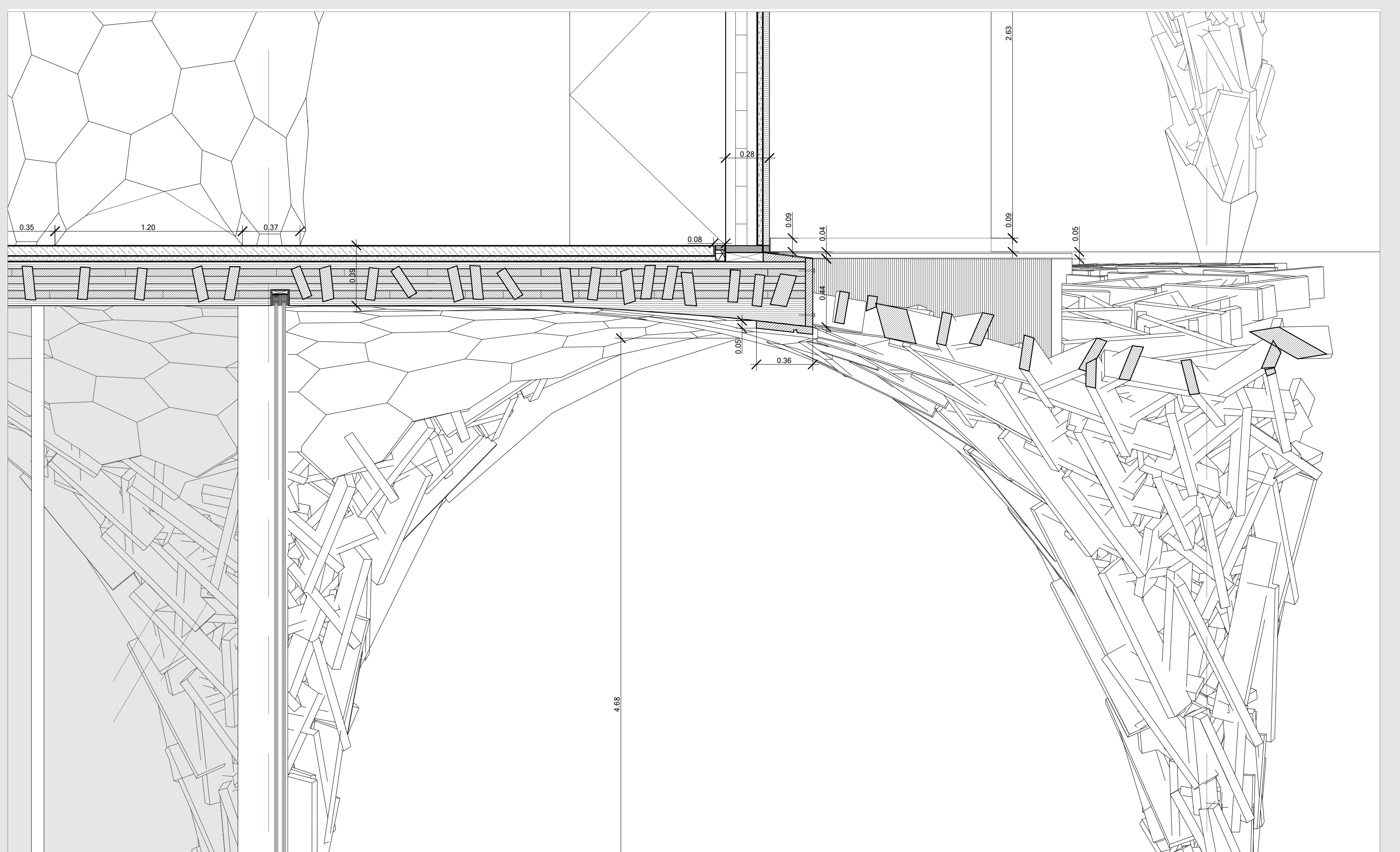
c - 1:20 Detail Section
