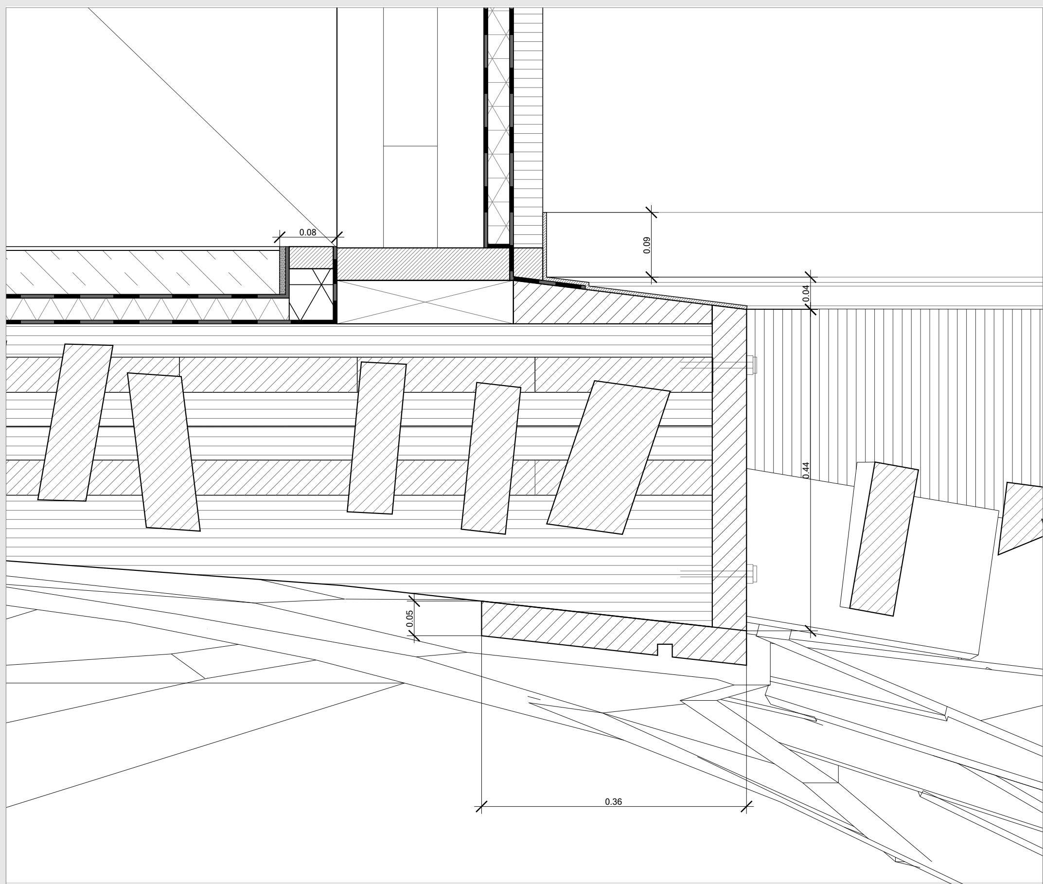
f - 1:50 Detail Section
