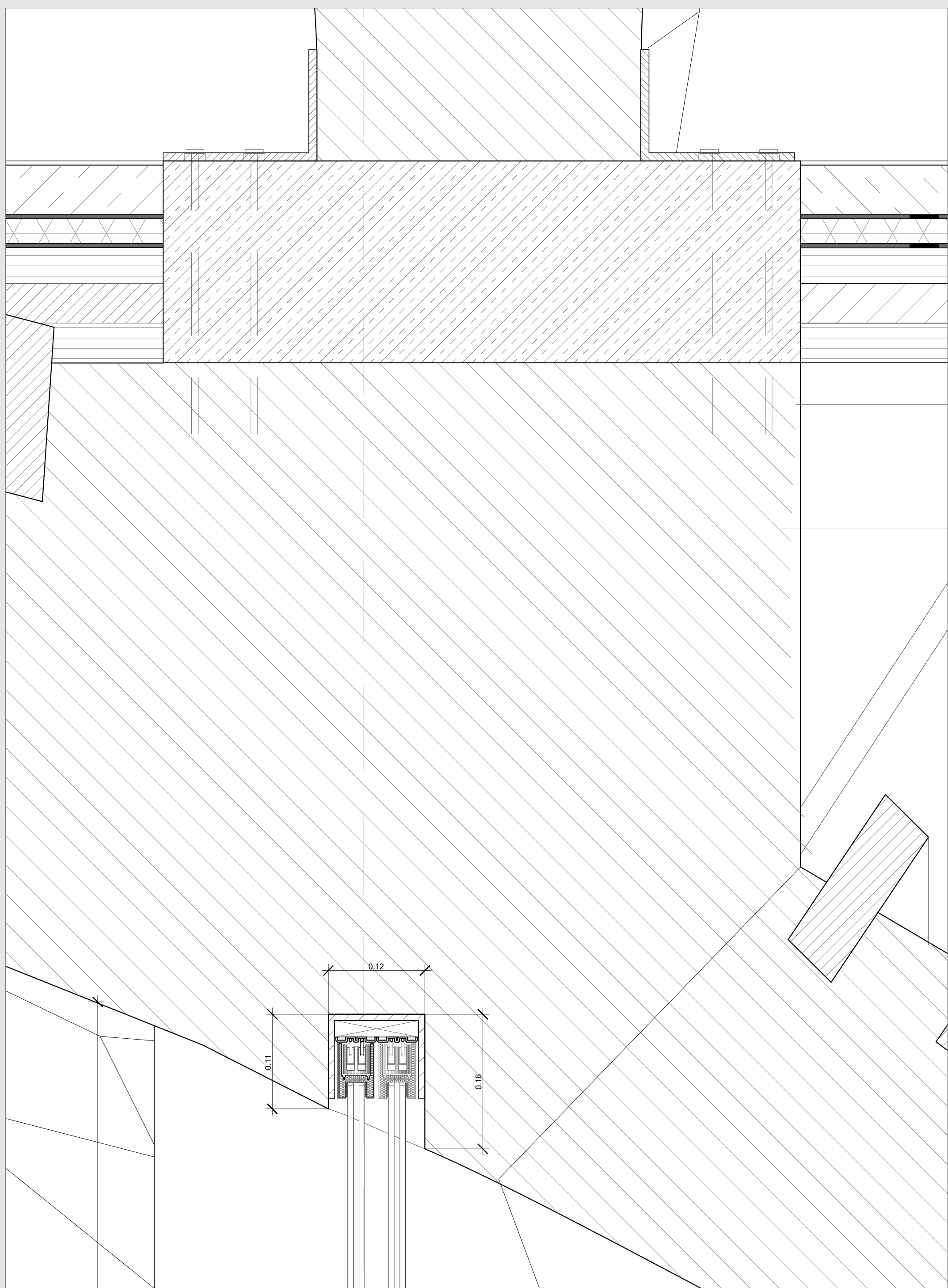
d - 1:50 Detail Section
