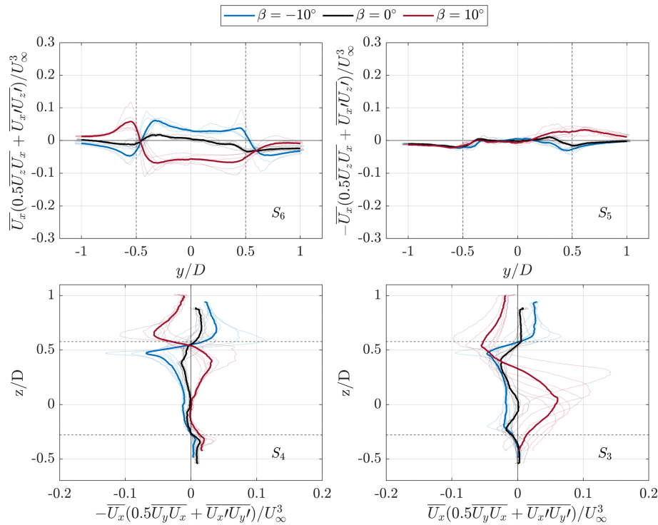
Figure 19. Axial and lateral components of the time-averaged streamwise MKE equation shown in Eq. (11) for the three pitch cases, normalized by the free stream flow component. Faint lines show the distributions along the control volume surfaces at each measurement location in the wake and thick solid lines show the mean across all positions. The vertical and horizontal dashed black lines show the edges of the control volume, as shown in Fig. 18. The labels toward the bottom right of the figures correspond to the control surfaces.
