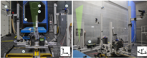
Figure 2. Experimental setup in the OJF from two different viewing angles. A visualization of the measurement plane (green triangle) is provided, along with a representation of the camera viewing direction. Main components: ① Camera 1, ② Camera 2, ③ field of view, ④ X-Rotor model, ⑤ OJF outlet, ⑥ traversing system, ⑦ laser.
