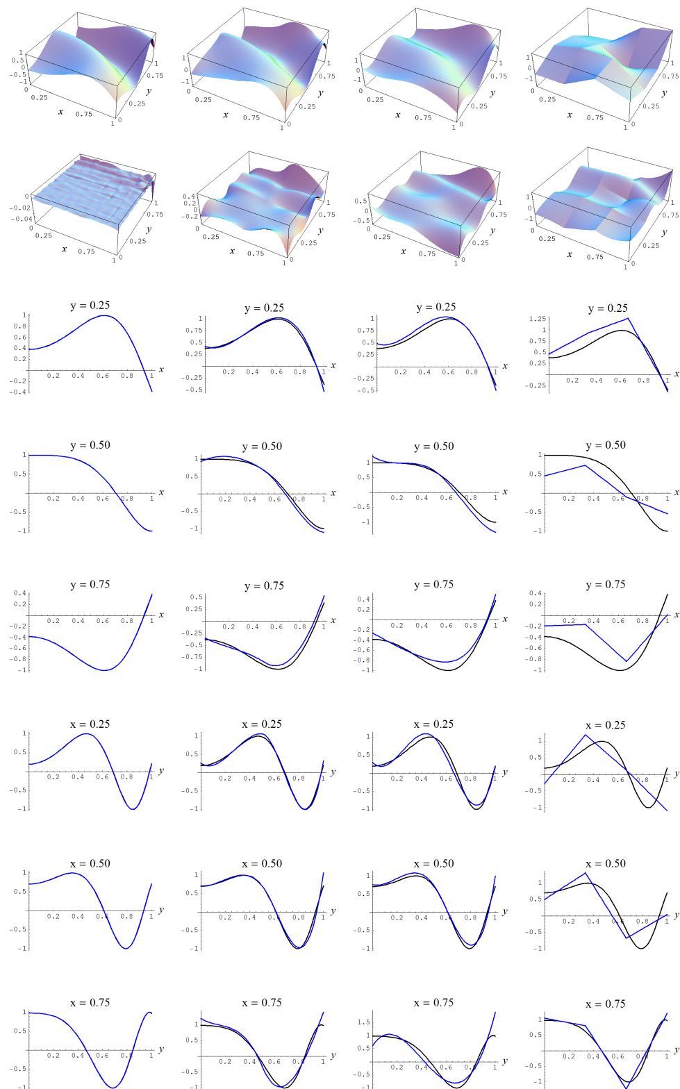
Figure A6. Sample size N = 5000 and C-spline models of target function (A2) are picked by the Ignorance, Manor, and BIC evidences, (135), (127), and (128), for different noise levels. Columns correspond with noise levels \sigma_n = 0, 1/2, 1 , and 2 , respectively. Rows correspond with spline model, residual of spline model relative to target function, and cross sections of spline model (blue) and target function (black).
