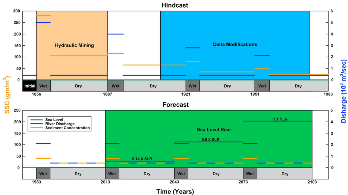
Figure 2. Schematization of the modeling timeline showing the hindcast (1856–1983) and forecast (1983–2103) along with the associated boundary conditions. The orange, blue and green lines represent the SSC, river discharge, and sea level, respectively. Sea level is increased for the forecast scenarios with 14%, 50%, and 100% of the total SLR imposed for 2013–2043, 2043–2073, and 2073–2103 periods, respectively. SLR = sea level rise.
