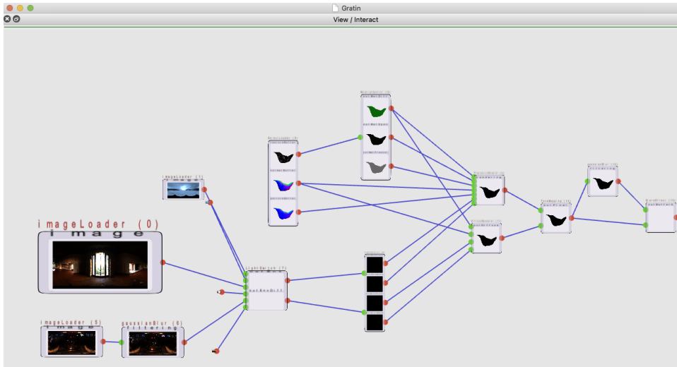
Figure 6.2: The node setups used in Gratin to implement the different material modes.
