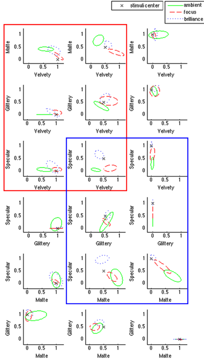
Figure 3.5: Interactions between each two of the reflectance modes. In each subplot, the matching results of 8 observers are fitted into one standard deviation bivariate ellipses. The black cross represents the weight combination of the stimulus in each subplot. In the top-left (red) block of six subplots, perceived velvetyness of the stimuli in comparison with the probe under office lighting decreases as the lighting changes from focus lighting to brilliance lighting to ambient lighting. In the middle-right (blue) block of another six subplots, perceived specularity of the stimuli in comparison with our probe decreases as the lighting changes from brilliance lighting to focus lighting to ambient lighting.
