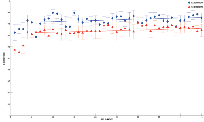
Figure 2.8: Average satisfaction ratings over all observers as a function of trial number, for Experiment 1 (blue) and Experiment 2 (red). Error bars of each data point represent one standard error of the sample mean.
