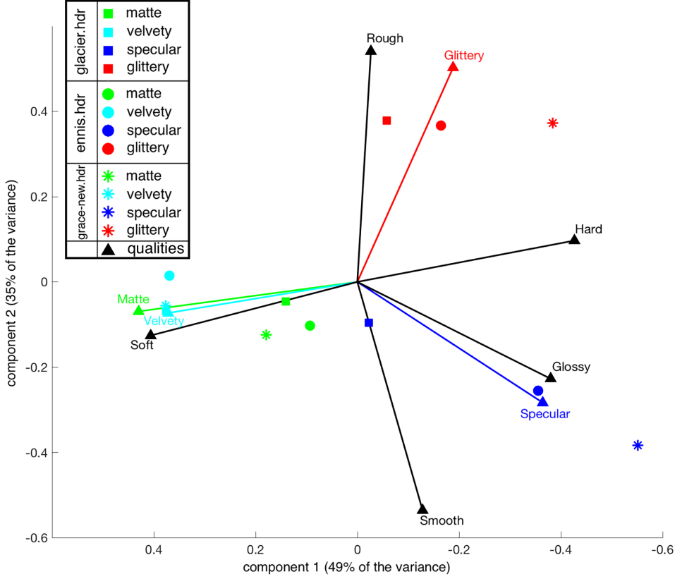
Figure 5.11: Results of the PCA for Experiment 2. The PCA was done on of the ratings per material quality per stimulus, with the medians determined across all observers and repetitions. The first component (x-axis) explains 49% of the variance. The second component (y-axis) explains 35% of the variance. The stimuli of the same material mode and corresponding qualities are colored the same, specifically matte in green, velvety in light blue, specular in indigo, and glittery in red. The other five qualities are colored black. The same shape marks the stimuli of the same lighting mode, specifically the Glacier light map as squares, the Ennis light map as circles, and the Grace-new light map as stars.
