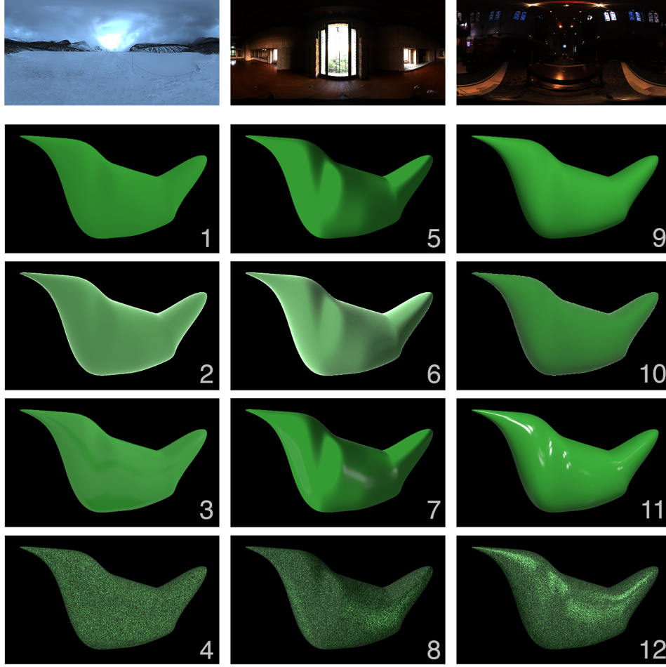
Figure 5.4: The stimuli of Experiment 2. From top to bottom, the first row shows the three lighting maps we selected to be the best representatives for the canonical lighting modes of the high resolution USC database. The second to the last rows represent the rendered matte, velvety, specular, and glittery material modes. From left to right, the three columns represent the materials under the Glacier, the Ennis, and the Grace-new illumination environments, respectively, as visualized in the first row. Compared to the initial Glacier environment, our version has been modified by filling in the black region originally found at the bottom of the image (which is due to the tripod base). The gammas of the images for the glittery mode (last row) were adjusted from 1.0 to 1.8 in order to make the features more visible in the printed version.
