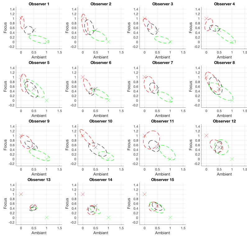
Figure 4.19: The bivariate plots for combination of ambient (green) and focus (red) lighting modes for each observer in Experiment 1. The subplots in each row are results for different lighting combinations. Different colors correspond to different lighting weight combinations in the stimuli, which are depicted by the crosses. The ellipses represent one standard deviation of bivariate normal distributions fitted to the data. Observer 1 to 4 are experienced observers. Observer 5 to 15 are inexperienced observers. Except for the last four observers, all performed well above chance if evaluated by the ratio r (Figure 4.4).
