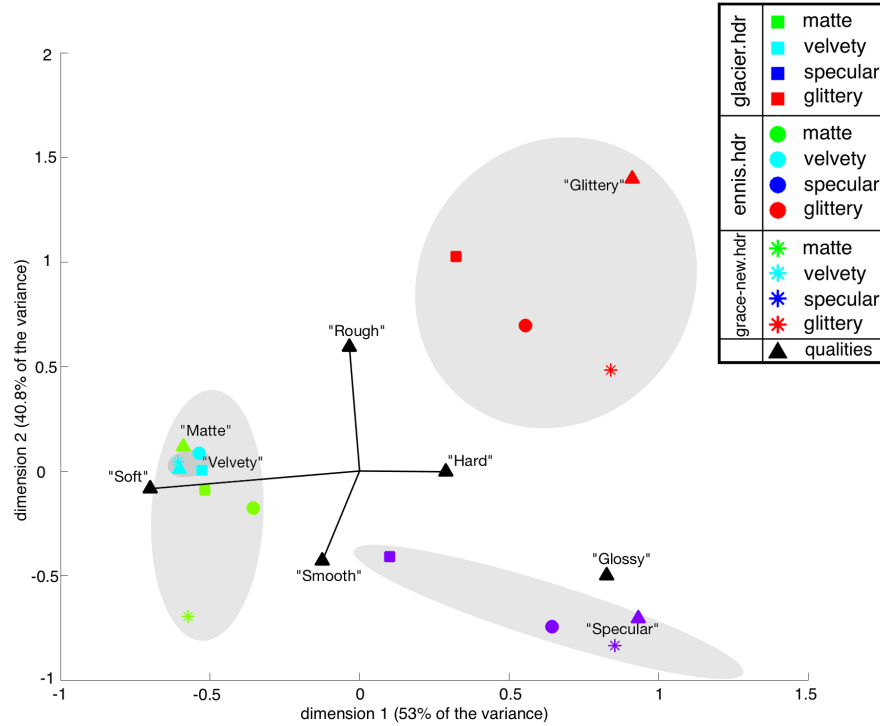
Figure 5.10: The visualization of the correspondence analysis results of the Y/N data for Experiment 2. The first dimension (x-axis) explains 53% of the variance. The second dimension (y-axis) explains 40.8% of the variance. The stimuli of the same material mode and their corresponding qualities are colored the same, specifically matte in green, velvety in light blue, specular in indigo, and glittery in red. The same shape marks the stimuli of the same lighting mode, specifically ambient light as squares, focus light as circles, and brilliance light as stars. The triangles represent the nine qualities that were tested in the Y/N question. The gray ellipses were intuitively drawn to show the distance between each stimulus and the quality. As in Figure 5.7, we connected the origin to soft, hard, rough, and smooth only to show that the two opponent pairs were orthogonal to each other.
