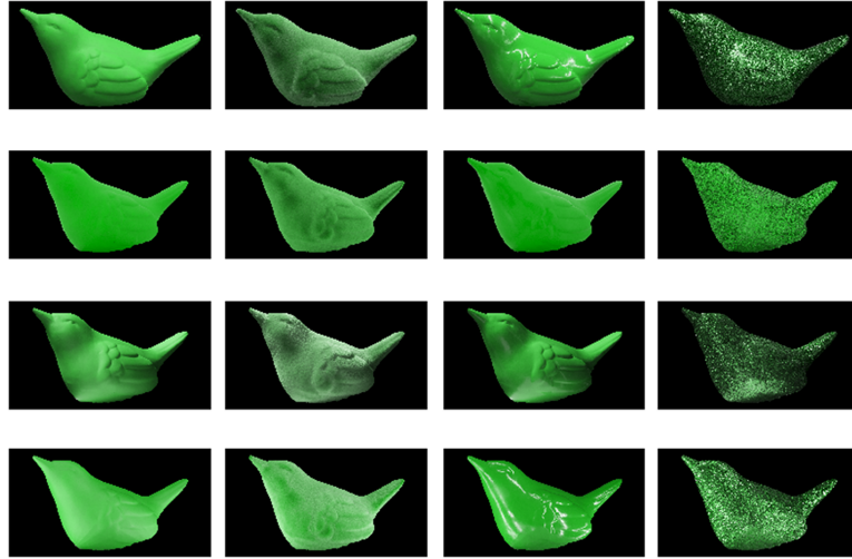
Figure 3.2: Basis images. From left to right each column shows a canonical reflectance mode, namely diffuse, asperity, forward and micro facet scattering, represented by matte, velvety, specular and glittery materials, respectively; From top to bottom the first row shows the probe basis images which were shot under generic office lighting, below which each row shows stimulus basis images for a canonical lighting mode, namely ambient lighting, focus lighting and brilliance lighting (from second to fourth row, respectively).
