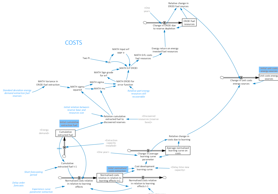
Figure 5. View of the costs sub-model
