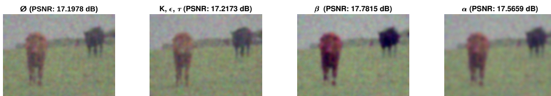
Figure 5. Example reconstruction results obtained from the denoising-reconstruction method for the different parameter settings for Example 8.2 described in subsection 8.4.3.
