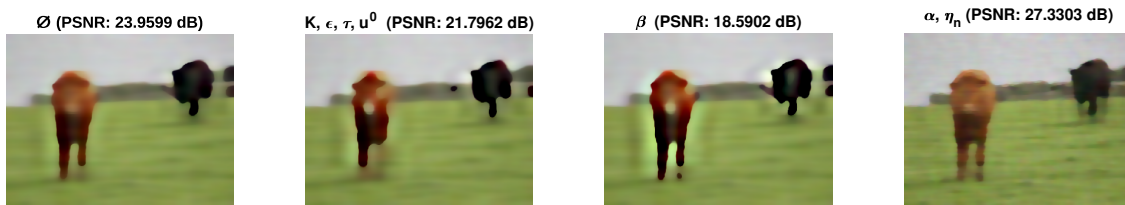
Figure 14. Example reconstruction results obtained from the deblurring-reconstruction method for the different parameter settings for Example 8.3 described in subsection 8.5.4.
