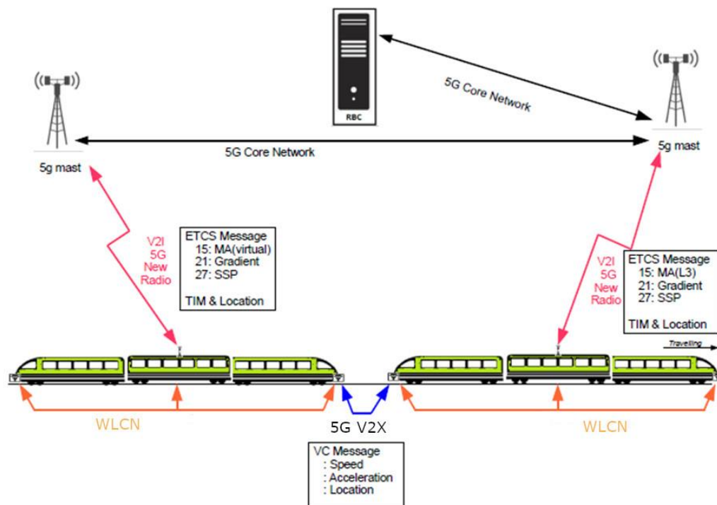
Figure 17: Virtual Coupling communication proposal for mainline railways
