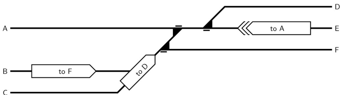
Figure 9: Trains blocked by a train stopping within a point zone
