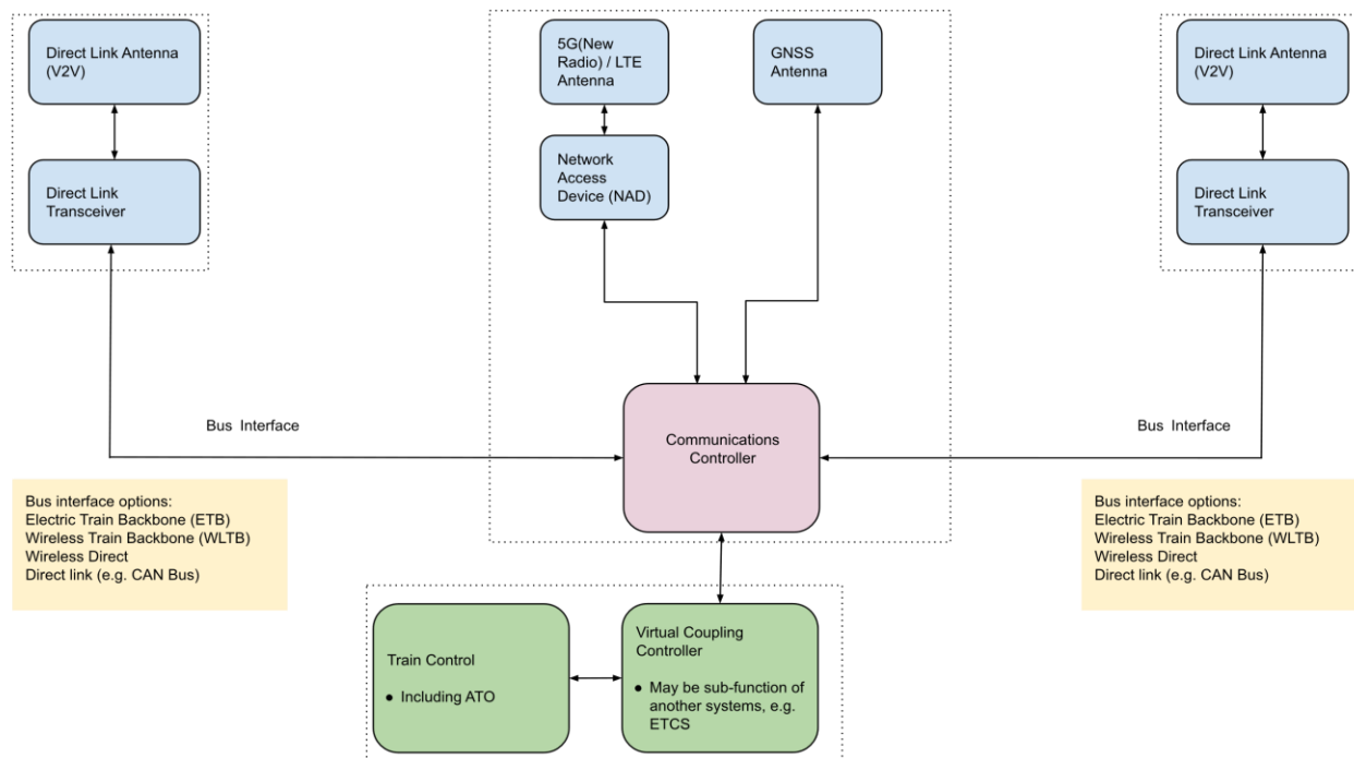
Figure 16: Virtual Coupling communication equipment architecture diagram
