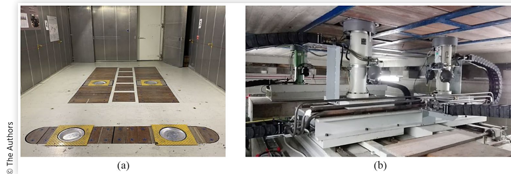
FIGURE 6 (a) Semi-anechoic chamber in which vehicle is placed on the 4-poster test rig; (b) room below the floor of the semi-anechoic chamber housing the actuators.
